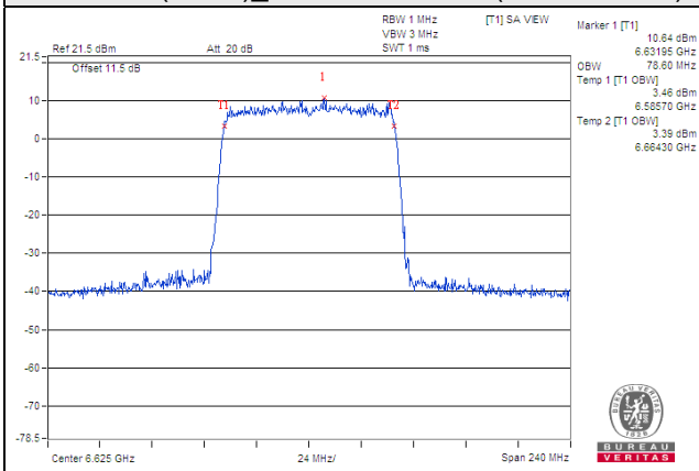
802.11ax (HE80)_Chain 0 / CH135 (U-NII-7 Band)
