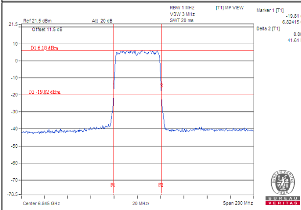
802.11ax (HE40)_Chain 1 / CH 179 (U-NII-7 Band)
