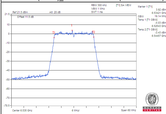
802.11ax (HE20)_Chain 0 / CH 117 (U-NII-7 Band)
