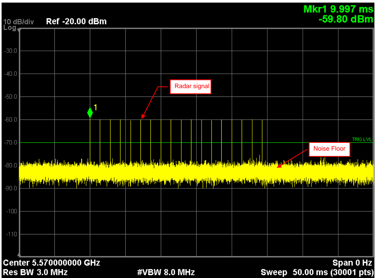
Radar Signal 0
