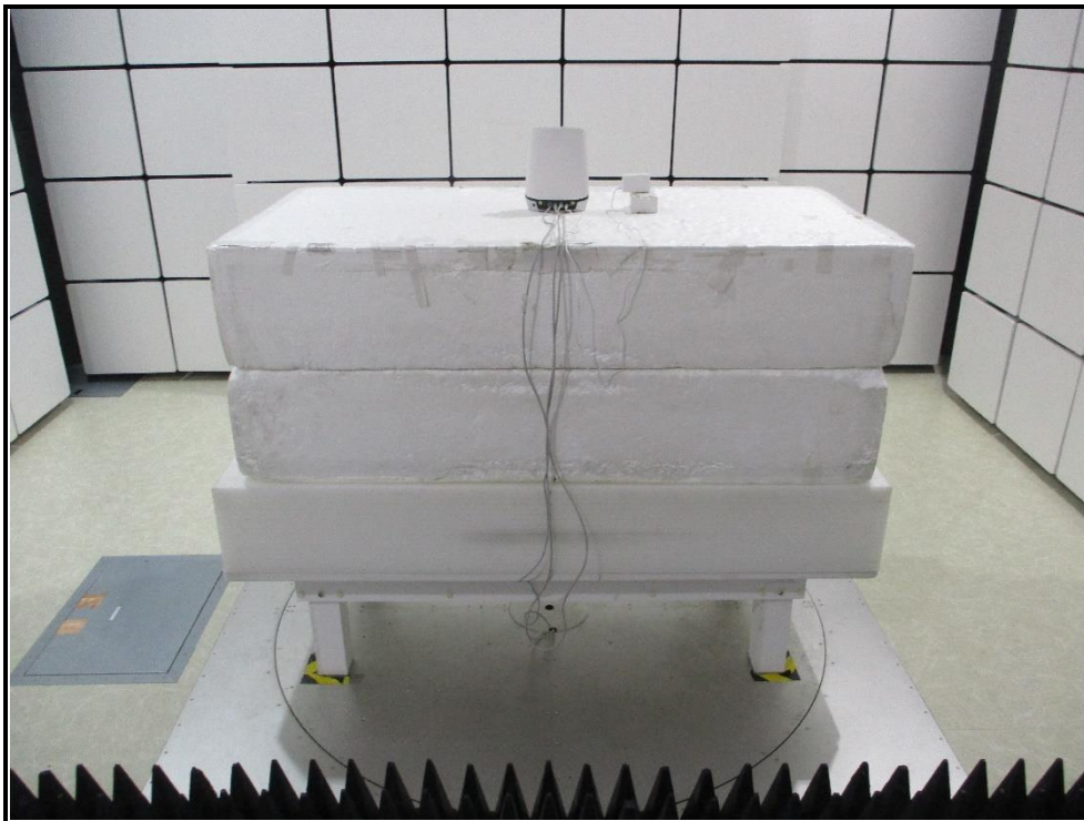
Internal Antenna
