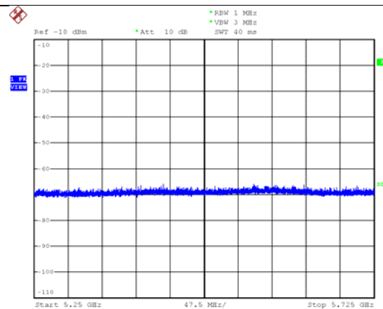
Client (UUT) no transmit on 802.11ax (HE40) mode
