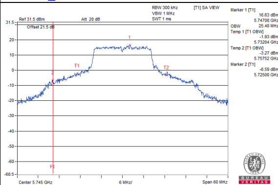
802.11a_Chain 1 / CH149
