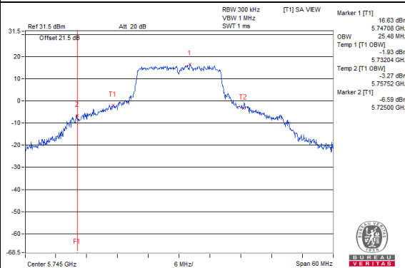
802.11a_Chain 1 / CH149
