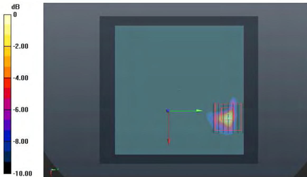
WLAN5.8G_802.11ac VHT80_Front Face_10mm_Ch155_Ant 4
