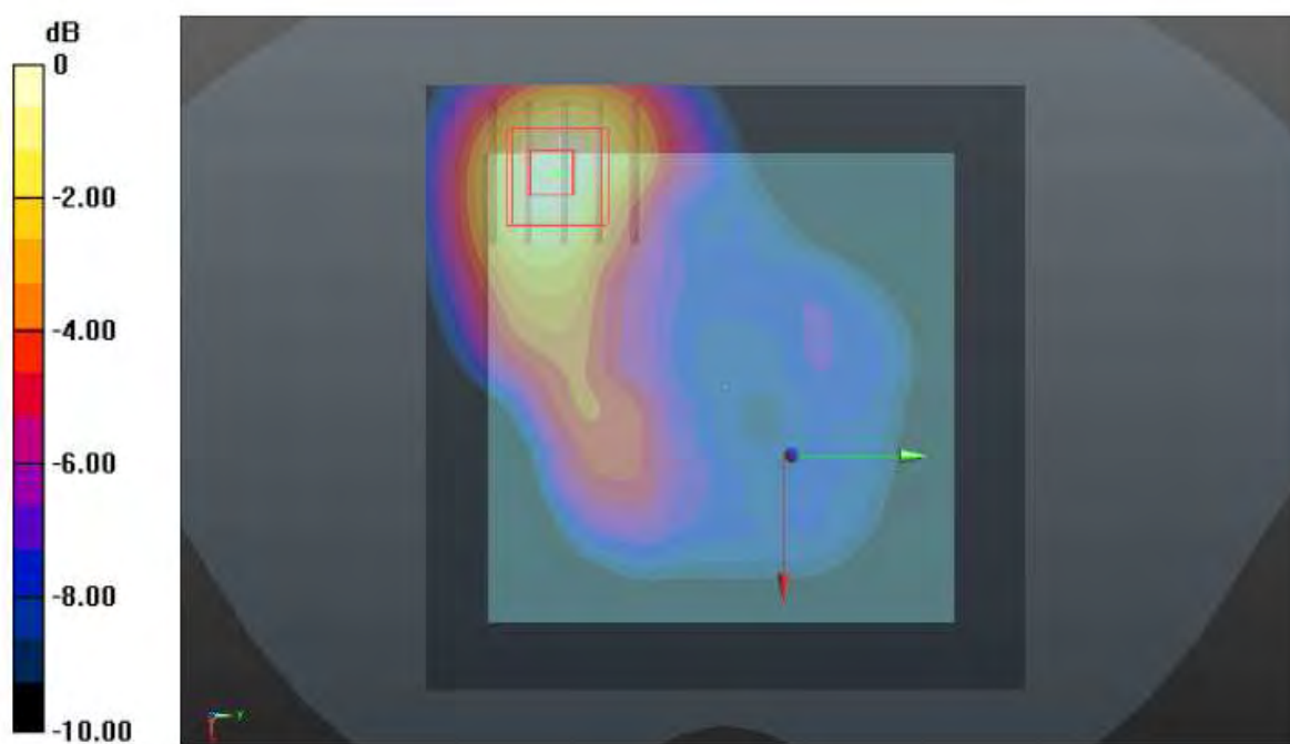
n66_DFT-S_QPSK_Front Face_10mm_Ch349000_1RB_OS53_Ant1_EN-DC_w
