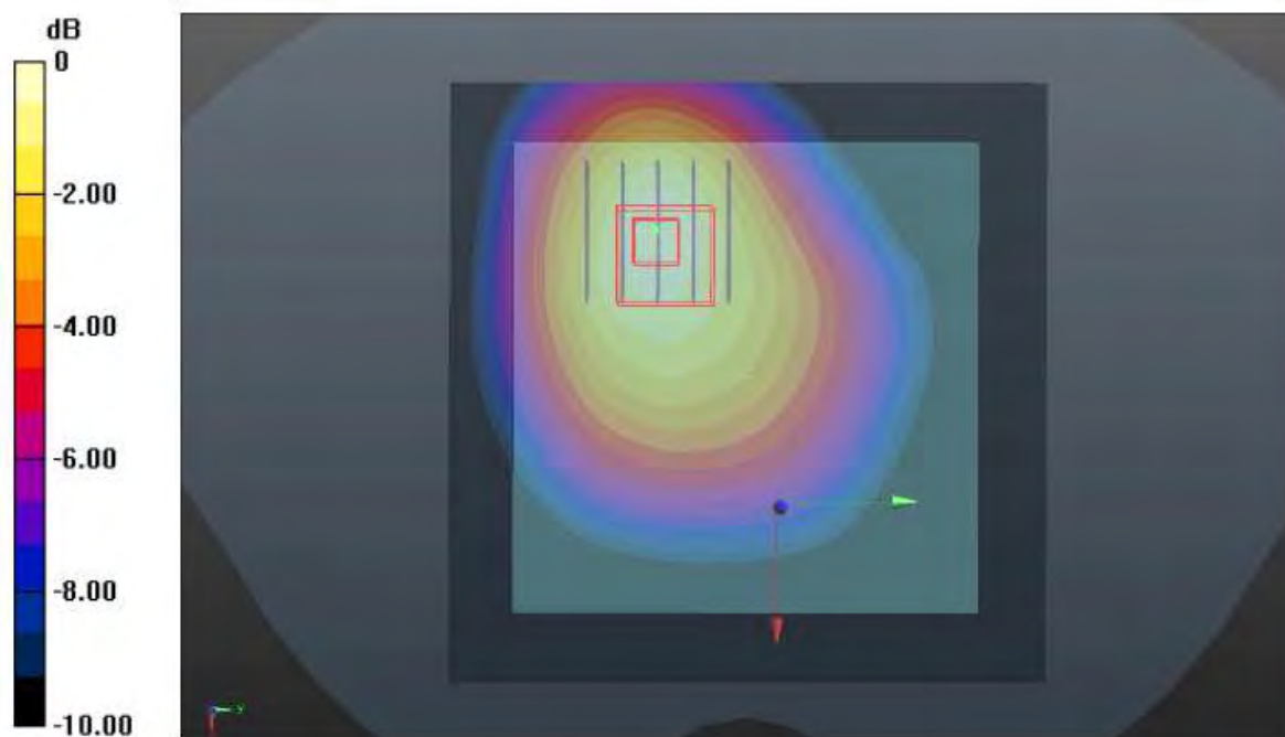
n66_DFT-S_QPSK_Front Face_10mm_Ch349000_1RB_OS53_Ant1_EN-DC_w
