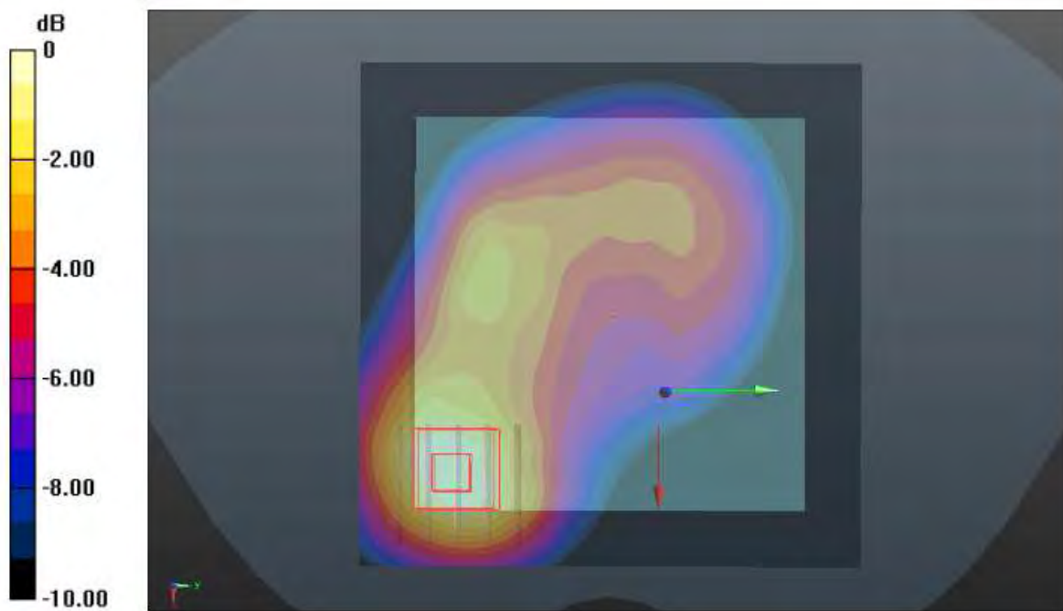
LTE 4_QPSK20M_Rear Face_10mm_Ch20175_1RB_OS50_Ant1
