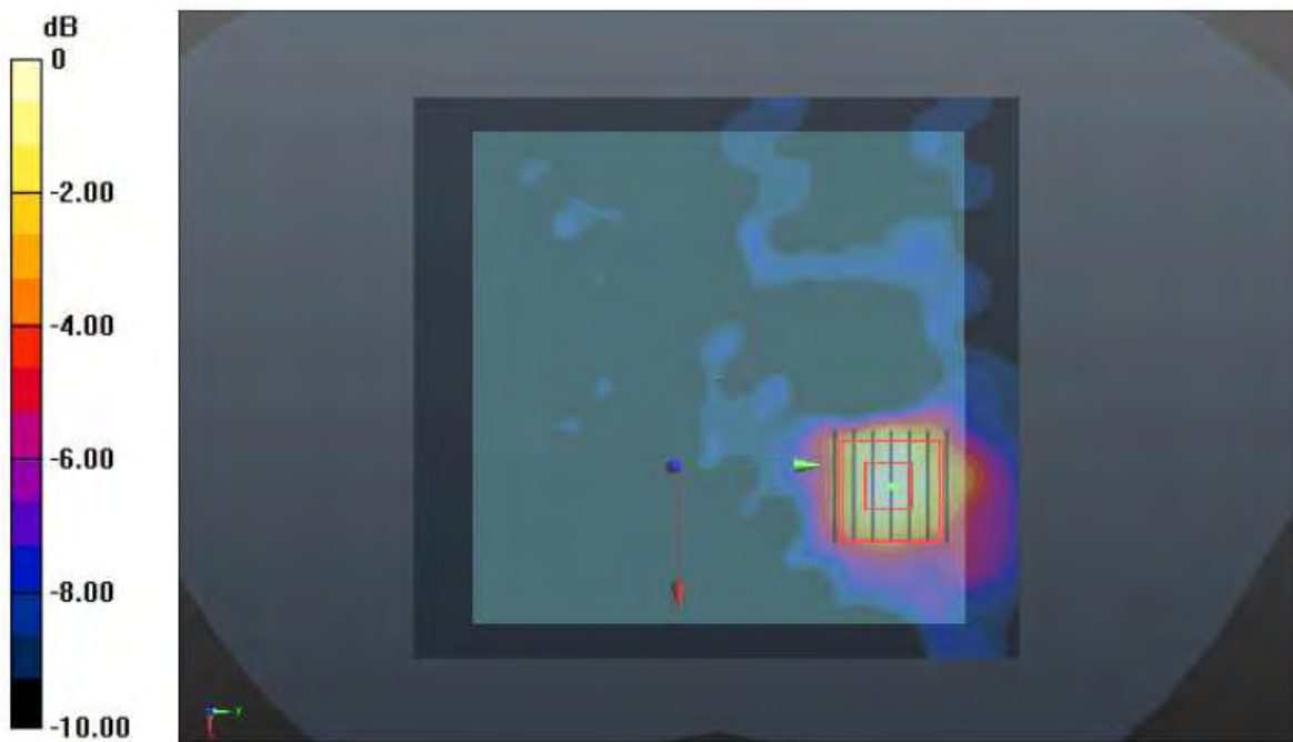
WLAN5.3G_802.11ac VHT80_Front Face_10mm_Ch58_Ant 4
