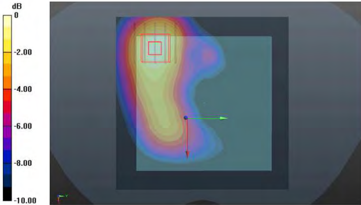
LTE 2_QPSK20M_Front Face_10mm_Ch18900_1RB_OS50_Ant1
