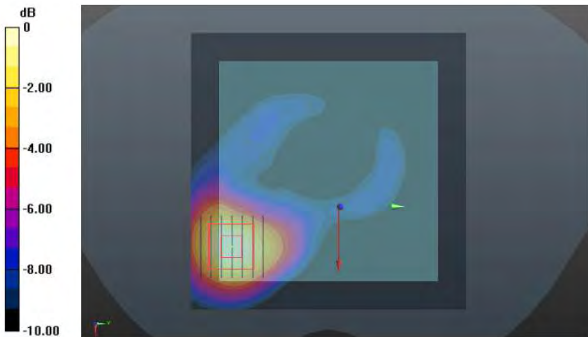
LTE 7_QPSK20M_Rear Face_10mm_Ch21350_1RB_OS0_Ant1
