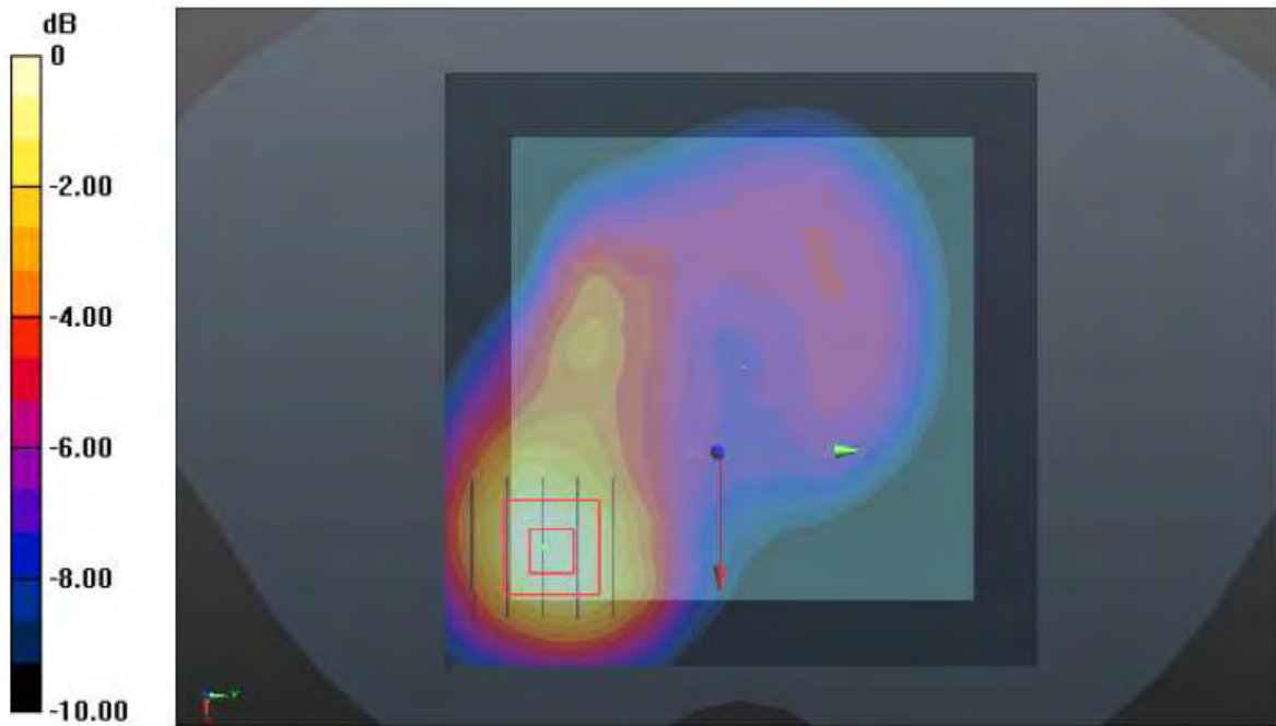
LTE 66_QPSK20M_Rear Face_10mm_Ch132572_1RB_OS50_Ant1
