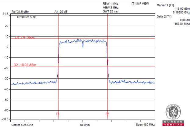
802.11ax (HE160)_Chain 2 / CH50
