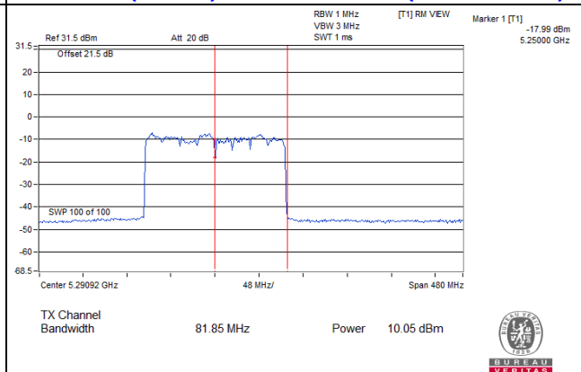
802.11ax (HE160)_Chain 2 / CH50 (U-NII-1 Band)
