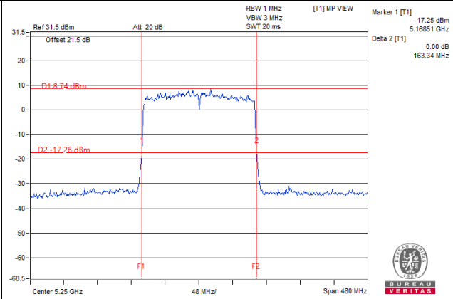
802.11ax (HE160)_Chain 1 / CH50
