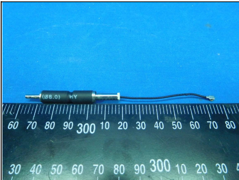
Antenna: 2.4GHz_Chain 1
