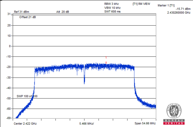
802.11ax (HE40)_Chain 3 / CH3
