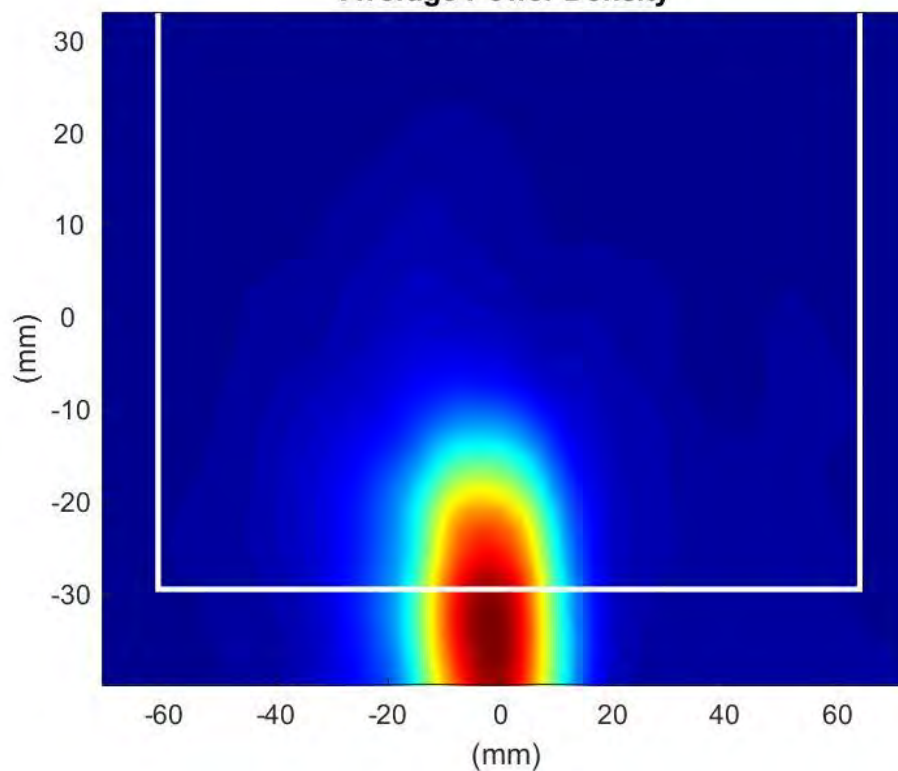
Phaser2 Beam:160 Surface:S2 Average Power Density
