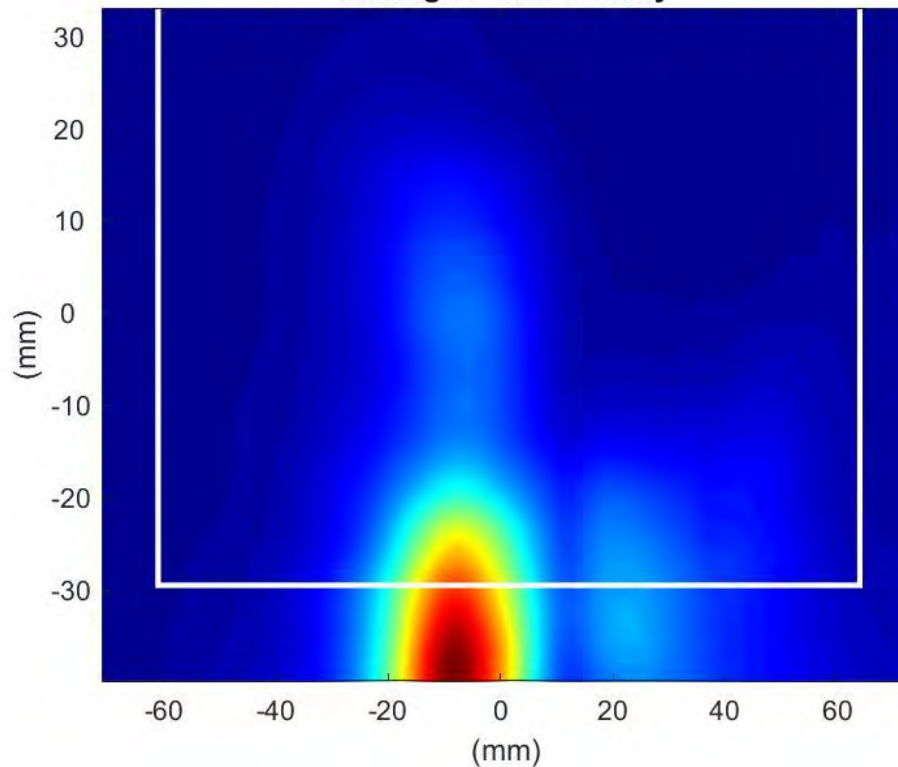
Phaser2 Beam:149 Surface:S1 Average Power Density
