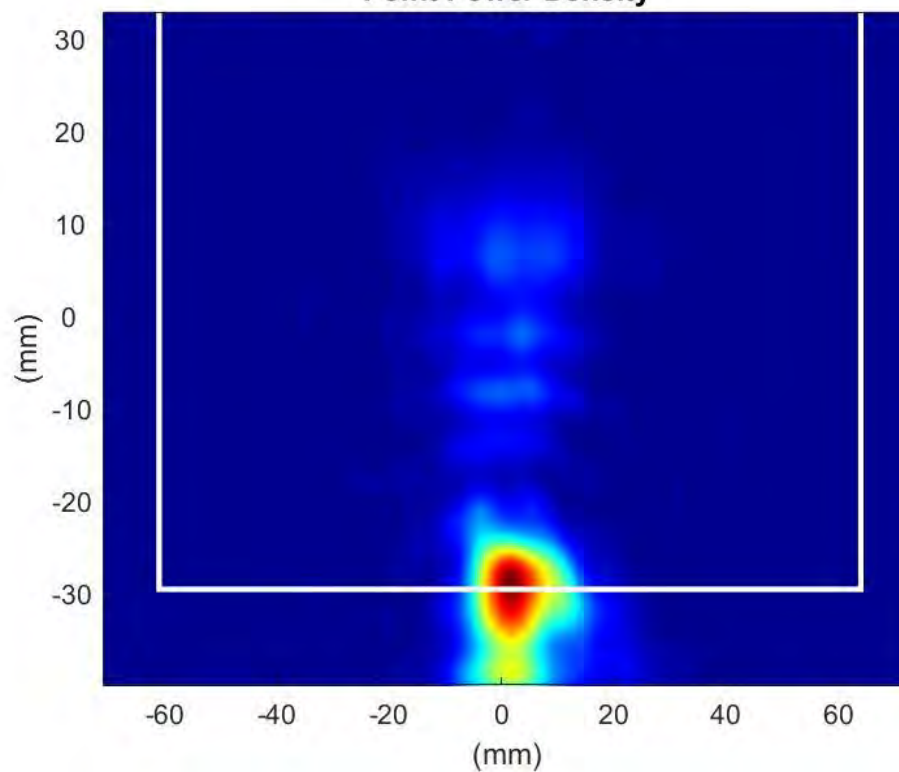
Phaser2 Beam:150 Surface:S1 Average Power Density
