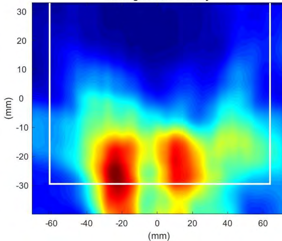
Phaser2 Beam:133 Surface:S2 Average Power Density
