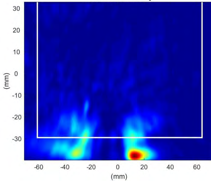
Phaser2 Beam:59 Surface:S1 Average Power Density
