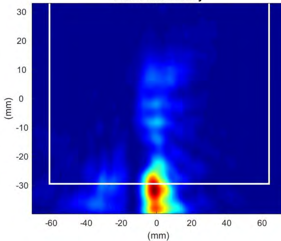
Phaser2 Beam:35 Surface:S1 Average Power Density
