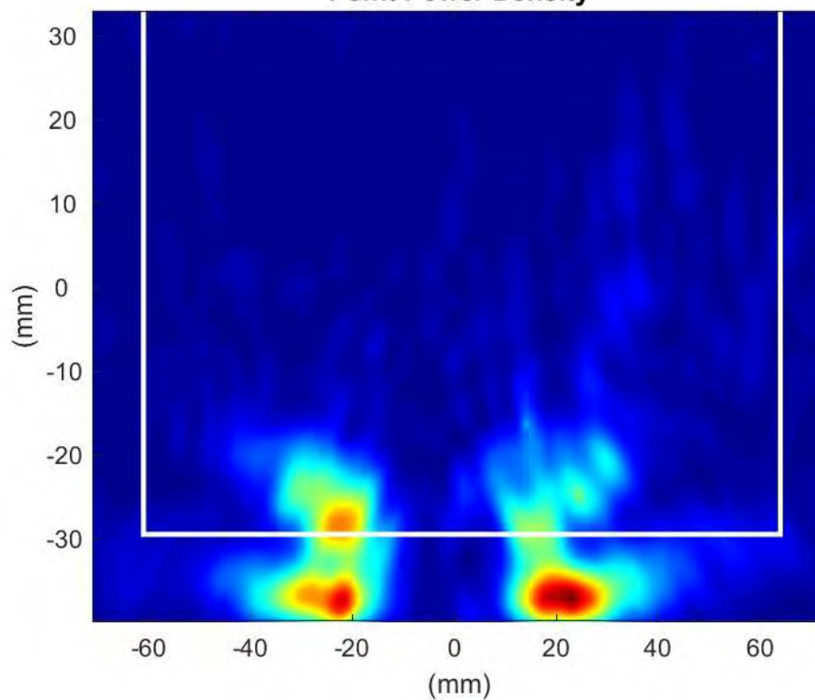
Phaser2 Beam:49 Surface:S1 Average Power Density
