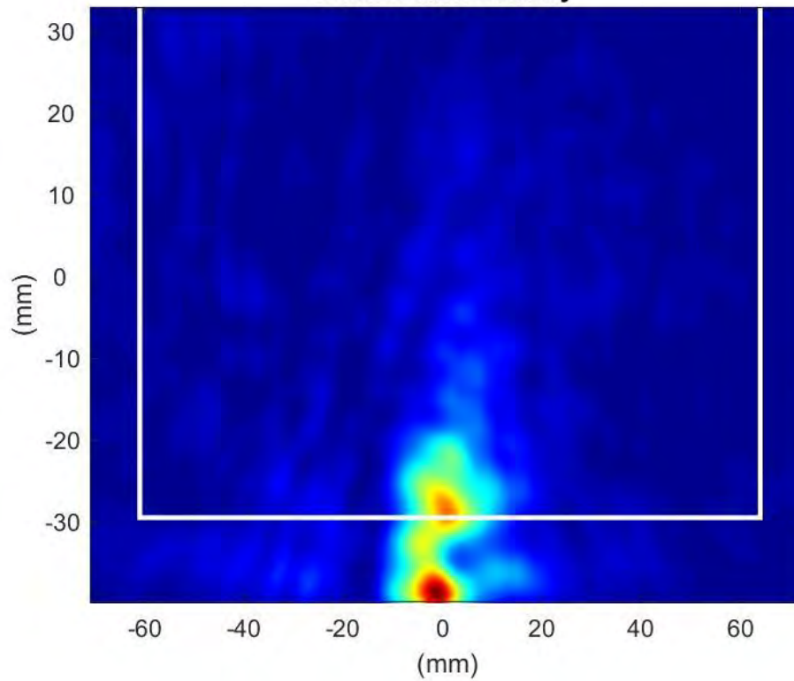
Phaser2 Beam:161 Surface:S1 Average Power Density
