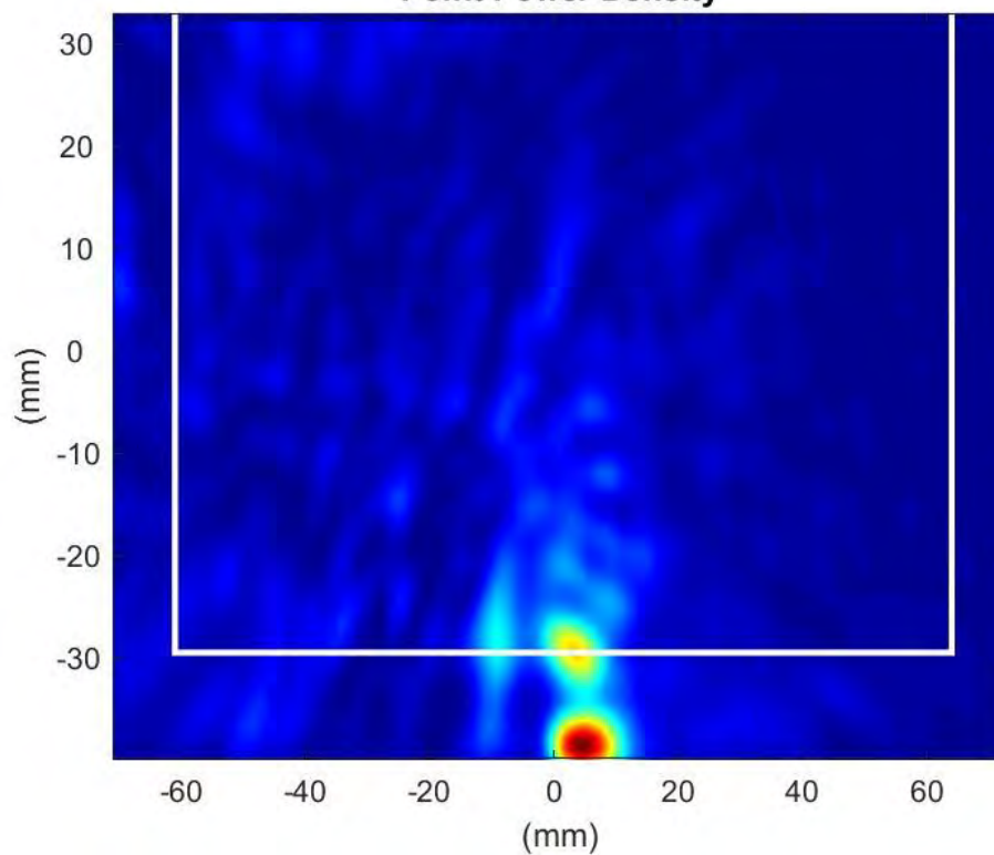
Phaser2 Beam:47 Surface:S1 Average Power Density
