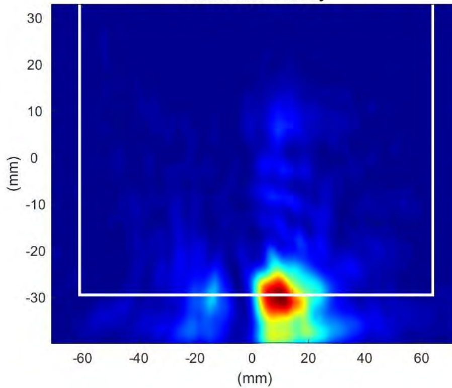
Phaser2 Beam:163 Surface:S1 Average Power Density
