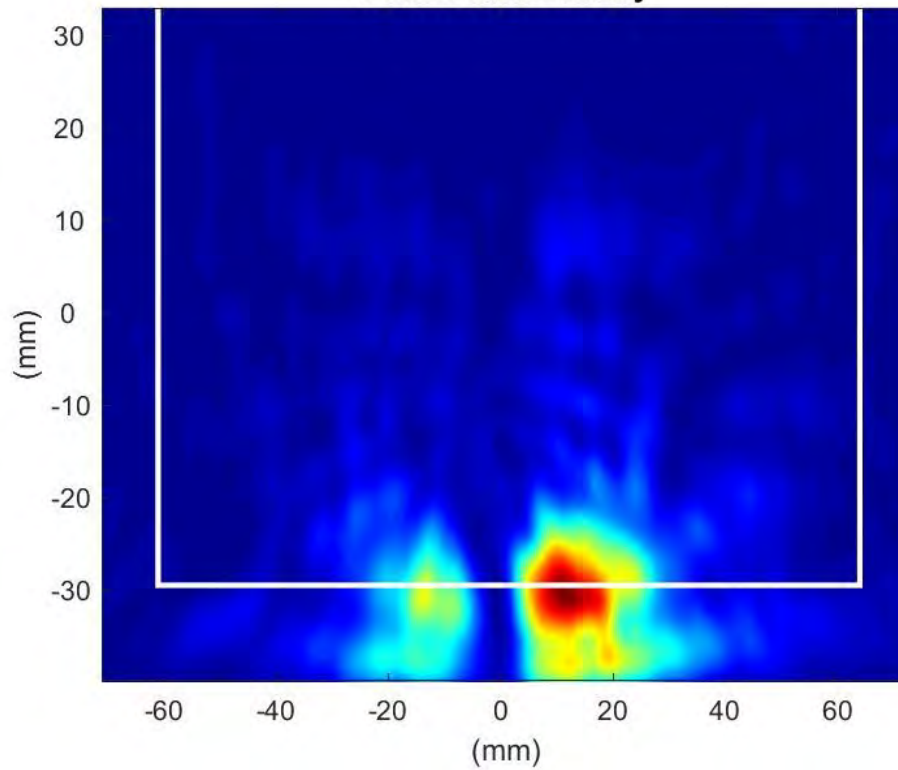
Phaser2 Beam:151 Surface:S1 Average Power Density
