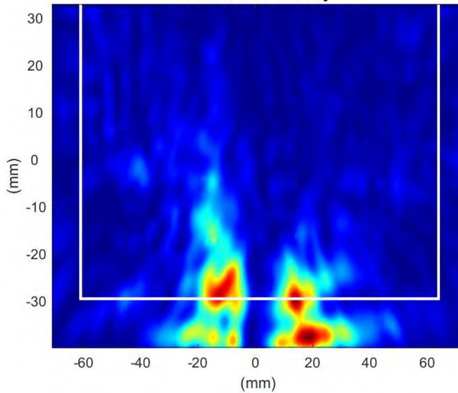
Phaser2 Beam:148 Surface:S1 Average Power Density
