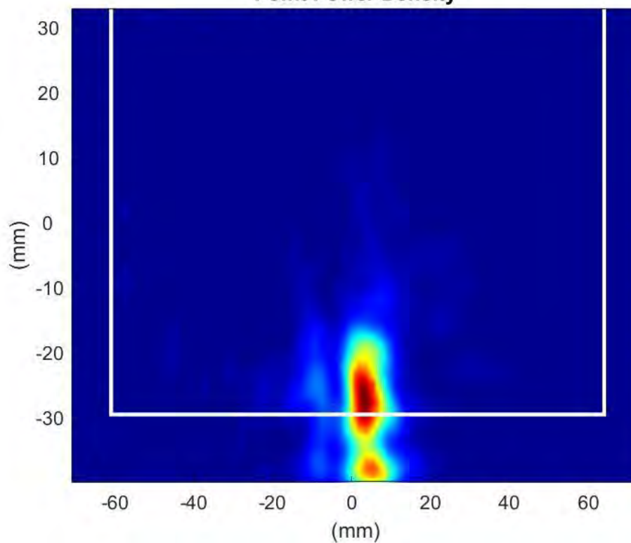
Phaser2 Beam:176 Surface:S2 Average Power Density
