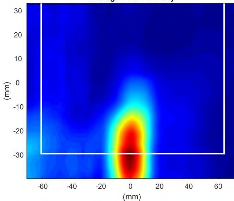
Phaser2 Beam:47 Surface:S2 Average Power Density
