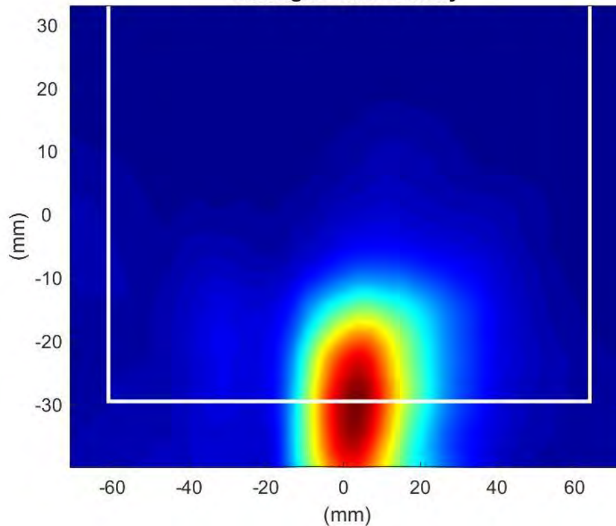
Phaser2 Beam:161 Surface:S2 Average Power Density
