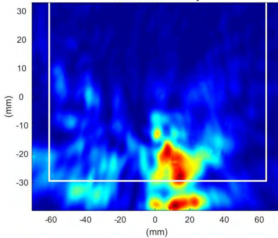
Phaser2 Beam:32 Surface:S2 Average Power Density
