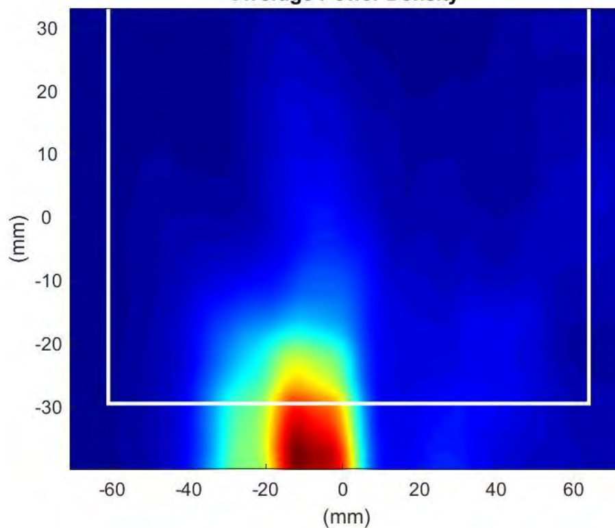
Phaser2 Beam:48 Surface:S1 Average Power Density
