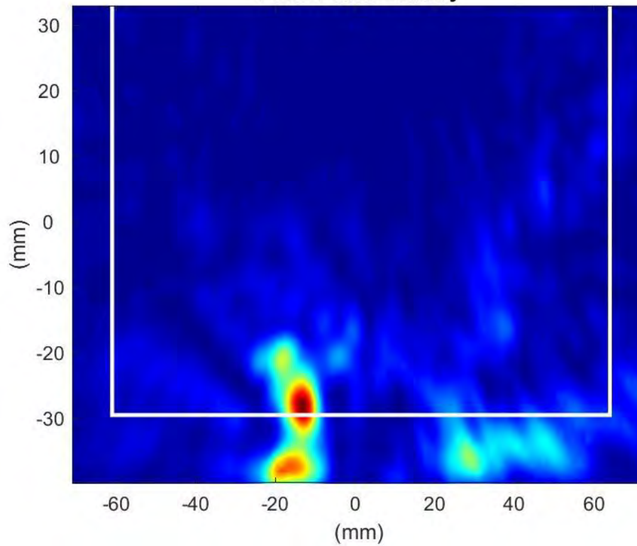
Phaser2 Beam:61 Surface:S2 Average Power Density
