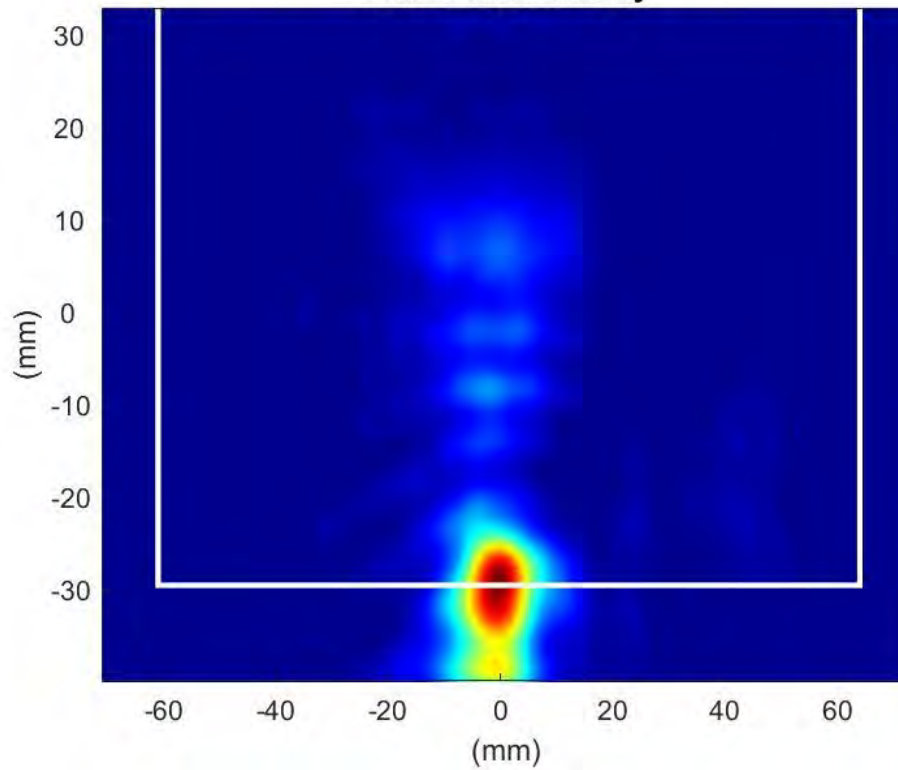
Phaser2 Beam:162 Surface:S1 Average Power Density
