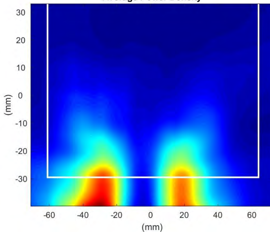
Phaser2 Beam:62 Surface:S2 Average Power Density
