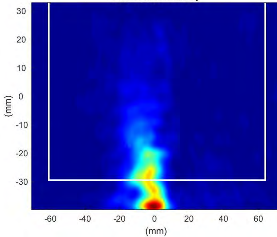
Phaser2 Beam:160 Surface:S1 Average Power Density
