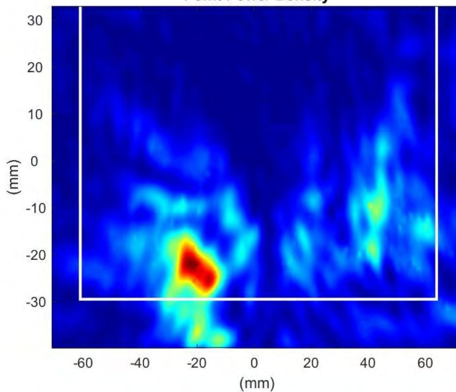
Phaser2 Beam:149 Surface:S2 Average Power Density
