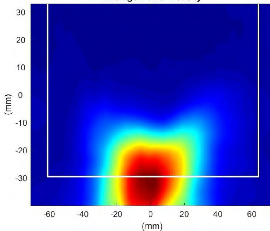
Phaser2 Beam:132 Surface:S2 Average Power Density
