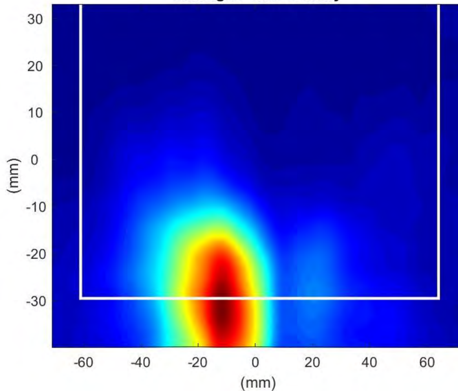
Phaser2 Beam:146 Surface:S2 Average Power Density
