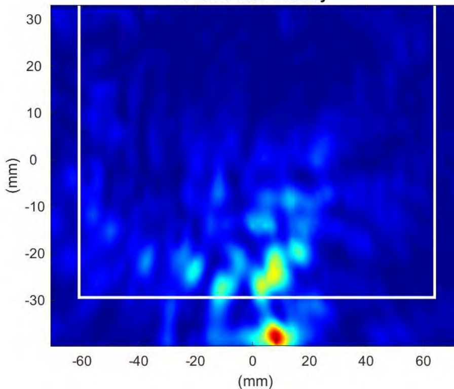
Phaser2 Beam:22 Surface:S2 Average Power Density
