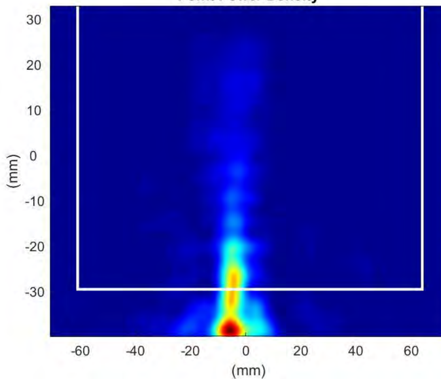
Phaser2 Beam:175 Surface:S1 Average Power Density
