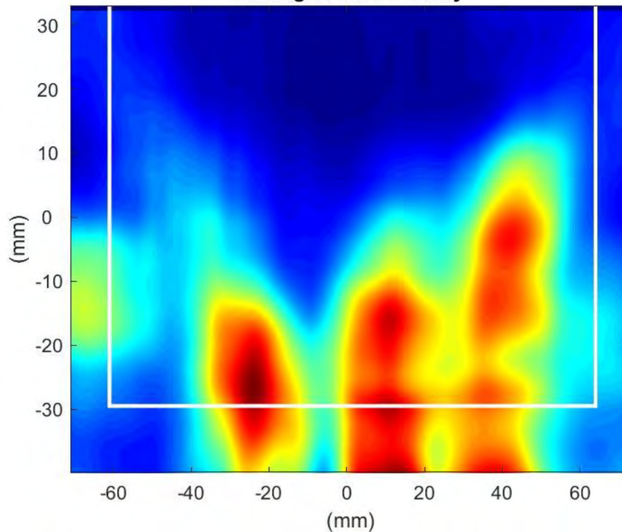
Phaser2 Beam:163 Surface:S2 Average Power Density
