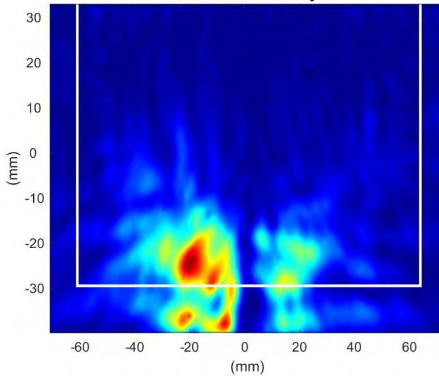
Phaser2 Beam:148 Surface:S2 Average Power Density
