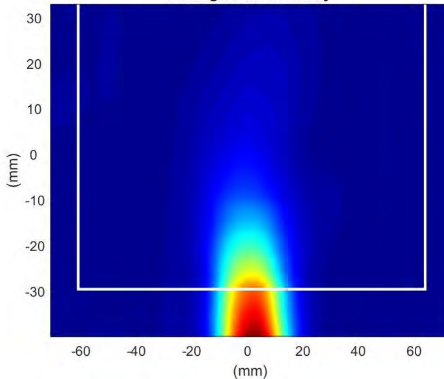
Phaser2 Beam:147 Surface:S1 Average Power Density
