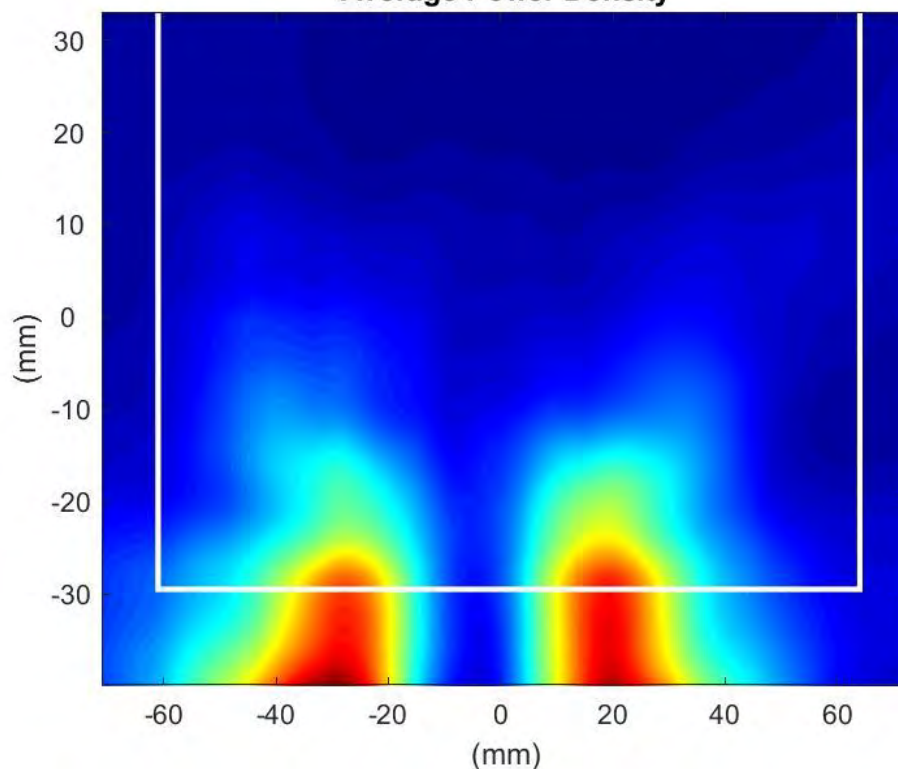
Phaser2 Beam:46 Surface:S2 Average Power Density
