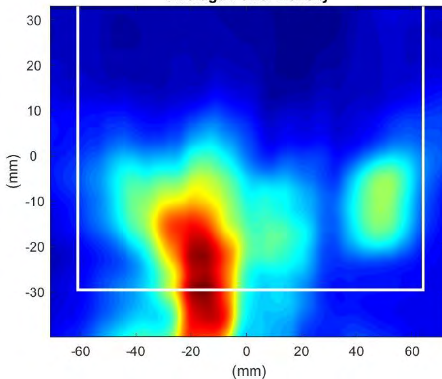
Phaser2 Beam:34 Surface:S2 Average Power Density
