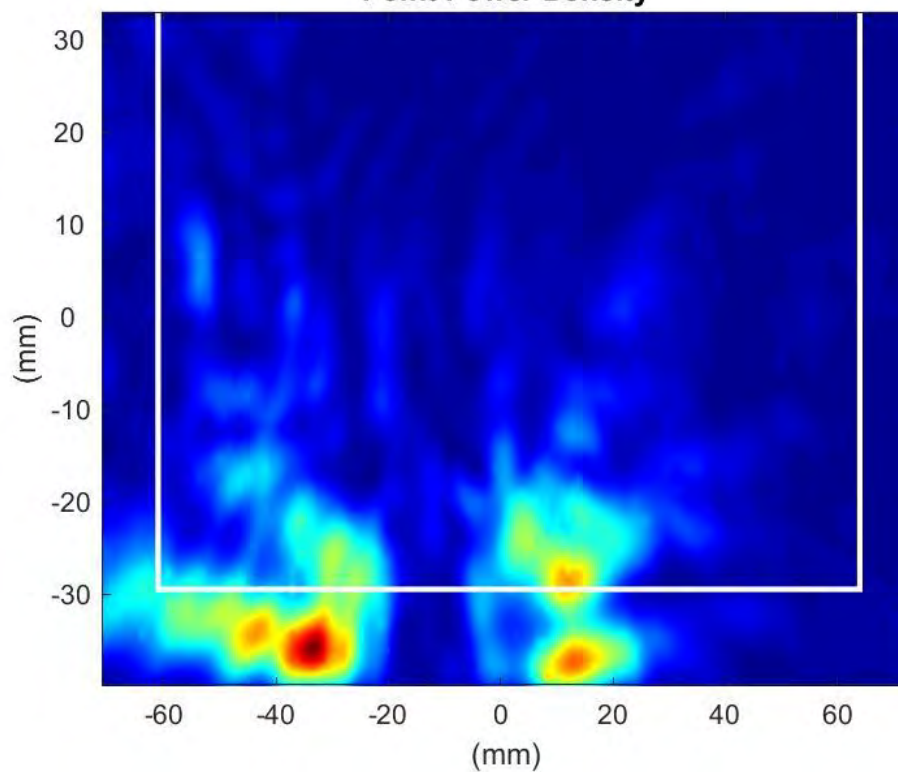
Phaser2 Beam:50 Surface:S2 Average Power Density
