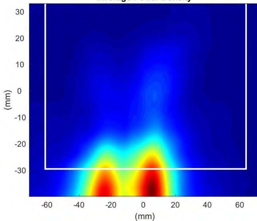
Phaser2 Beam:23 Surface:S1 Average Power Density
