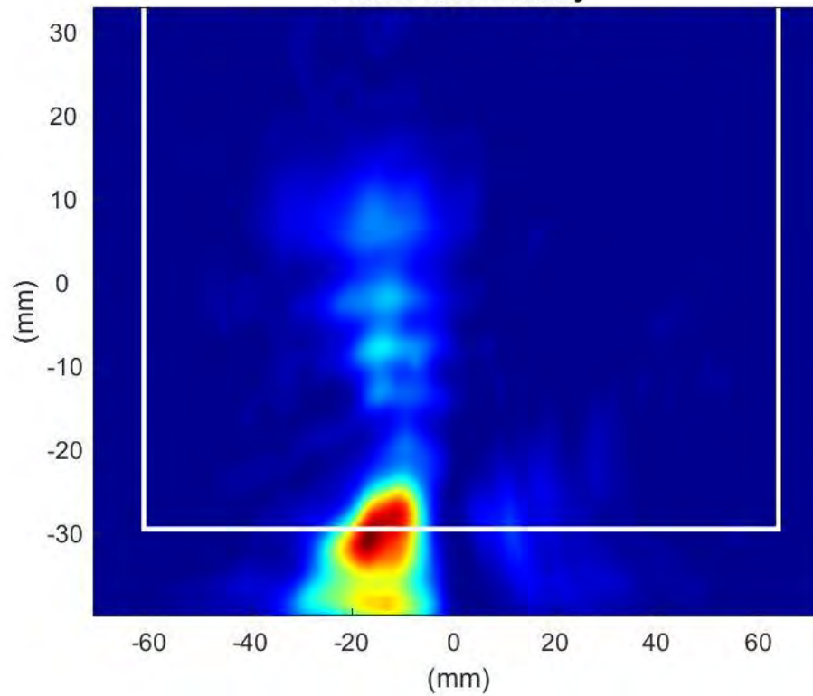
Phaser2 Beam:34 Surface:S1 Average Power Density
