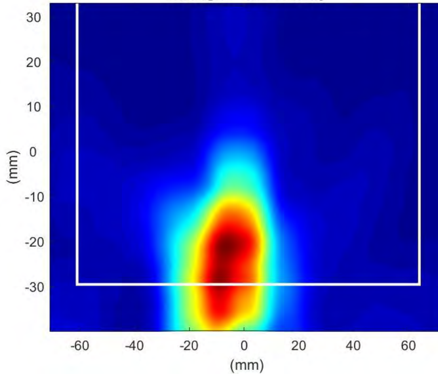
Phaser2 Beam:60 Surface:S2 Average Power Density
