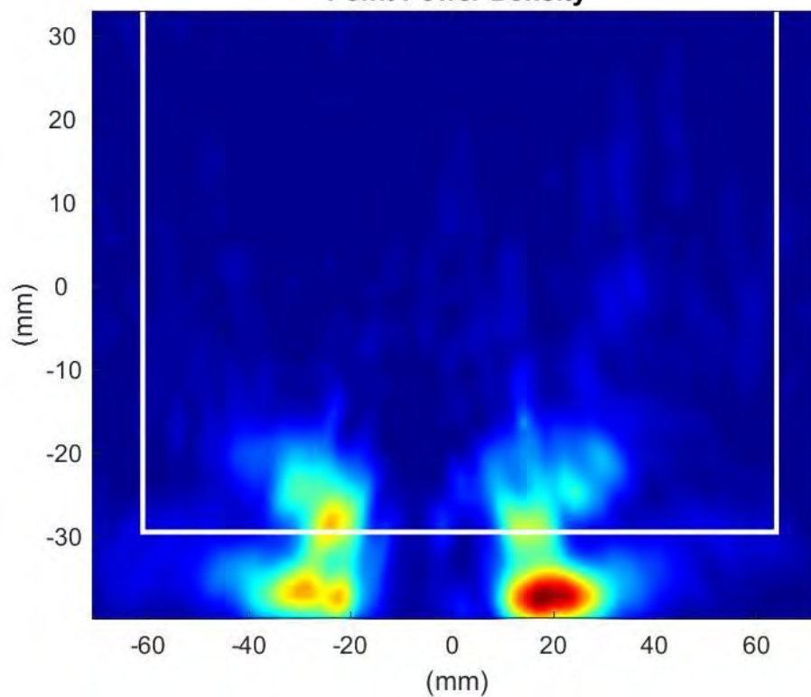
Phaser2 Beam:46 Surface:S1 Average Power Density
