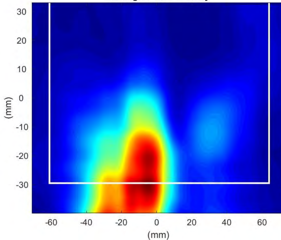
Phaser2 Beam:48 Surface:S2 Average Power Density
