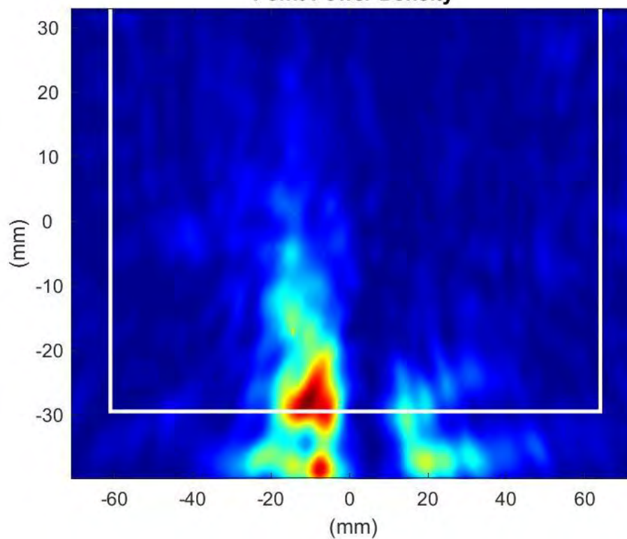
Phaser2 Beam:146 Surface:S1 Average Power Density
