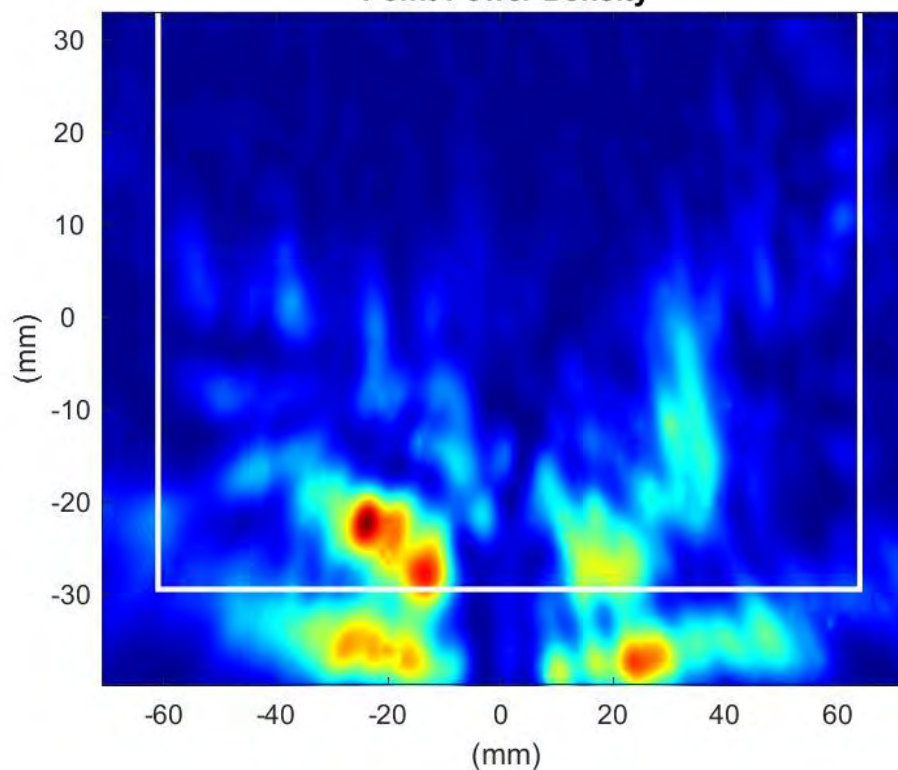
Phaser2 Beam:33 Surface:S2 Average Power Density
