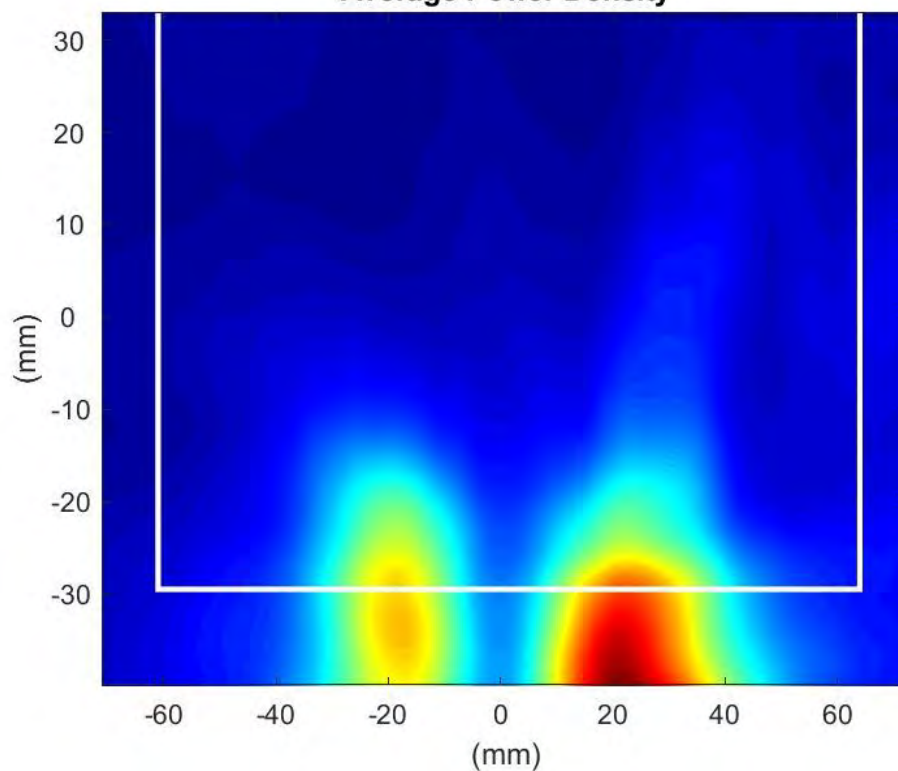
Phaser2 Beam:33 Surface:S1 Average Power Density
