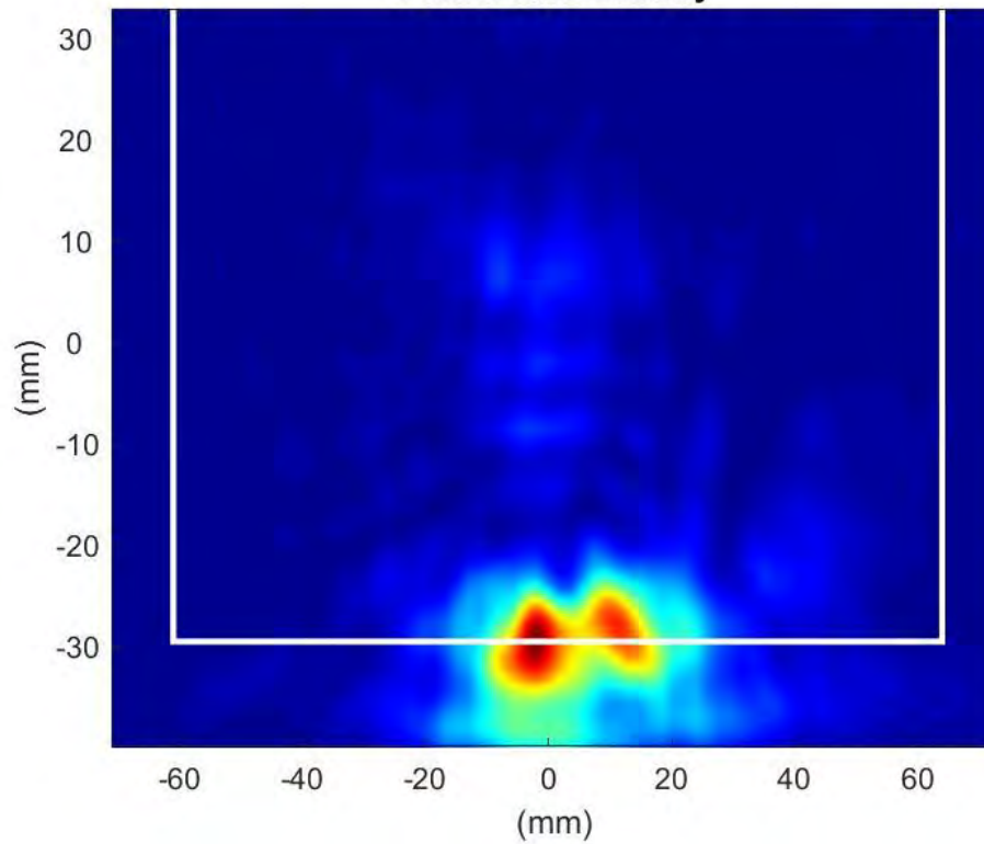
Phaser2 Beam:133 Surface:S1 Average Power Density
