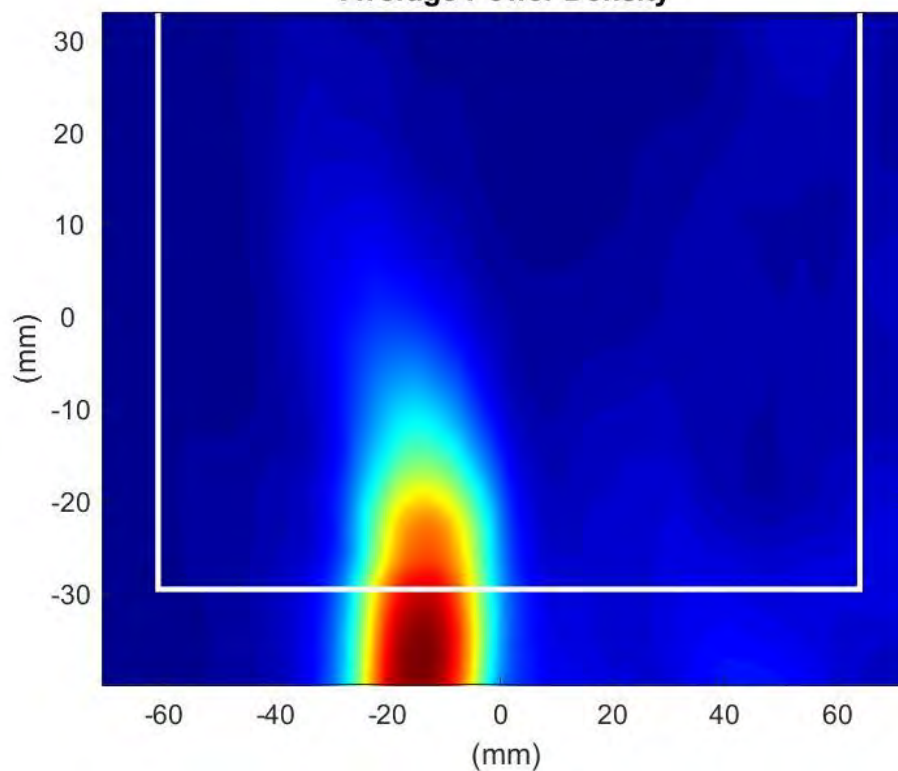
Phaser2 Beam:174 Surface:S1 Average Power Density
