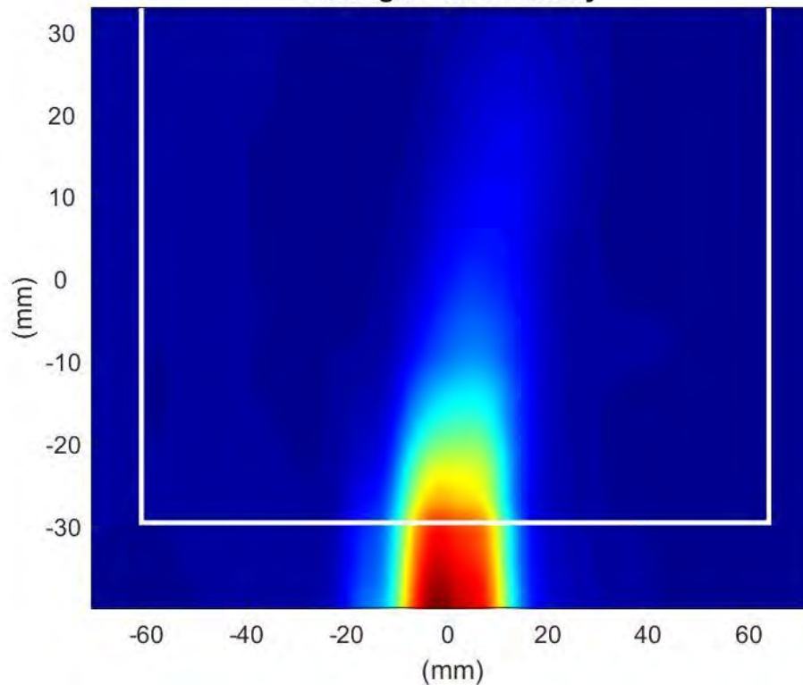
Phaser2 Beam:176 Surface:S1 Average Power Density
