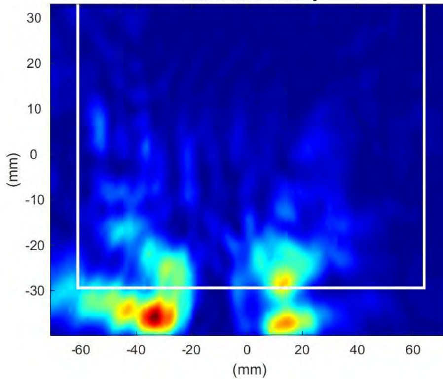
Phaser2 Beam:59 Surface:S2 Average Power Density
