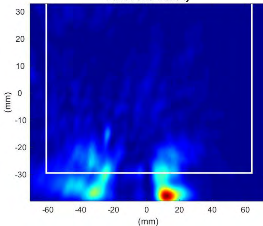
Phaser2 Beam:50 Surface:S1 Average Power Density
