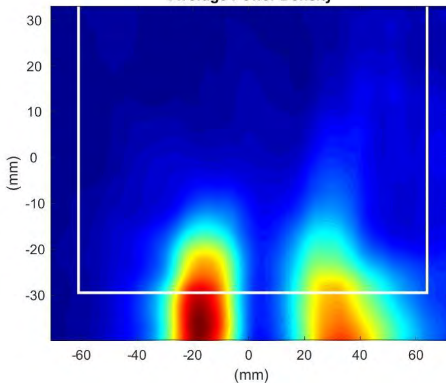
Phaser2 Beam:61 Surface:S1 Average Power Density
