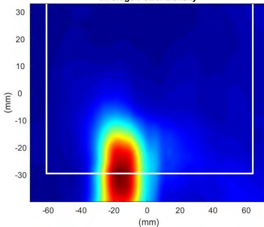
Phaser2 Beam:174 Surface:S2 Average Power Density
