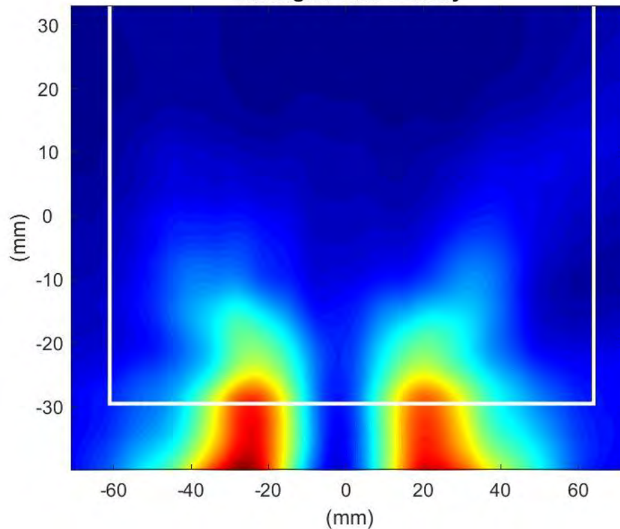
Phaser2 Beam:49 Surface:S2 Average Power Density
