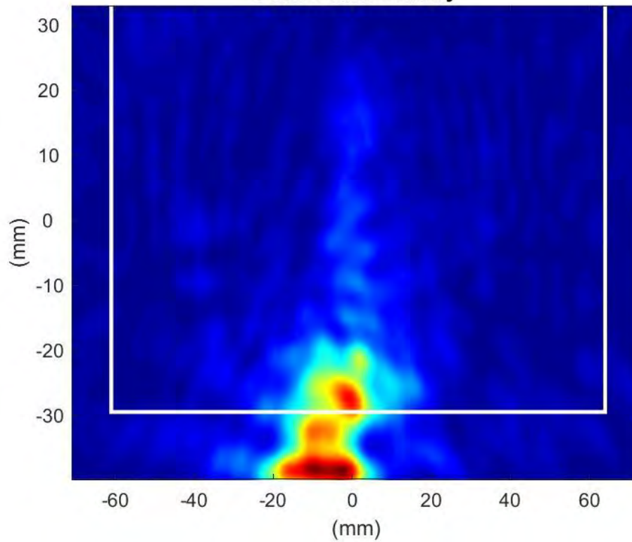
Phaser2 Beam:132 Surface:S1 Average Power Density
