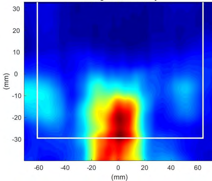
Phaser2 Beam:150 Surface:S2 Average Power Density
