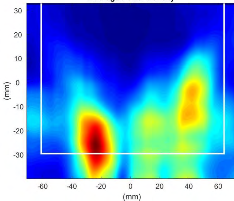
Phaser2 Beam:151 Surface:S2 Average Power Density
