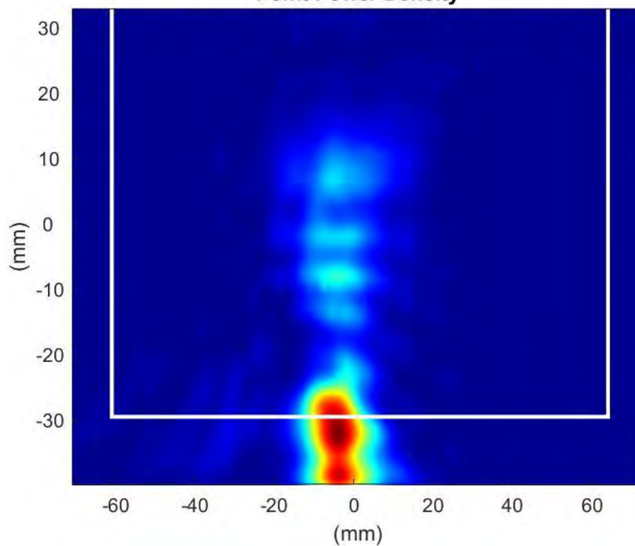
Phaser2 Beam:22 Surface:S1 Average Power Density
