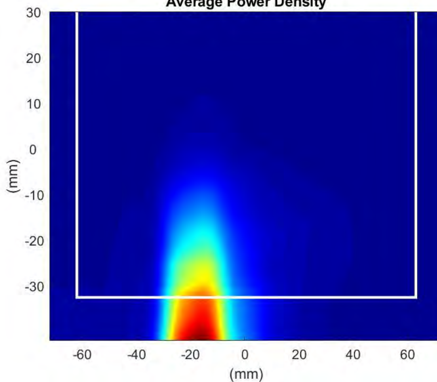
Phaser1 Beam Pair:37-166 Surface:S2 Average Power Density
