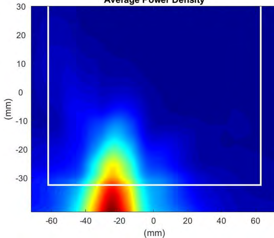
Phaser1 Beam Pair:27-154 Surface:S2 Average Power Density
