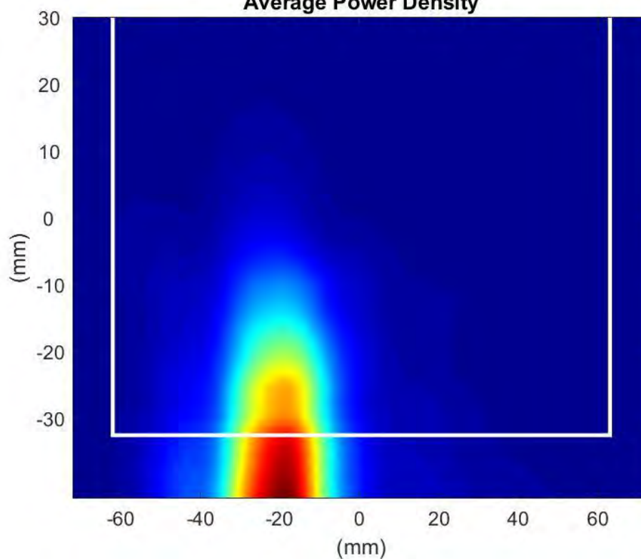
Phaser1 Beam Pair:52-180 Surface:S2 Average Power Density
