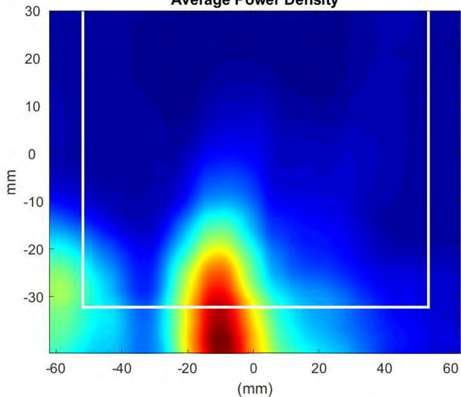
Phaser0 Beam Pair:43-169 Surface:S2 Average Power Density
