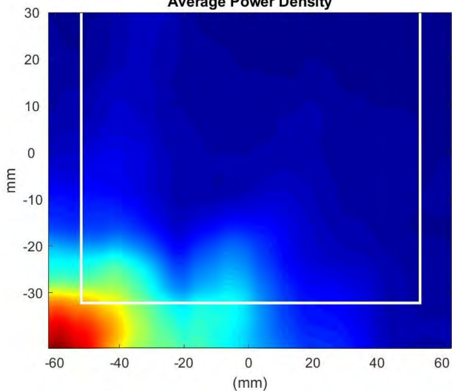
Phaser0 Beam Pair:17-145 Surface:S1 Average Power Density
