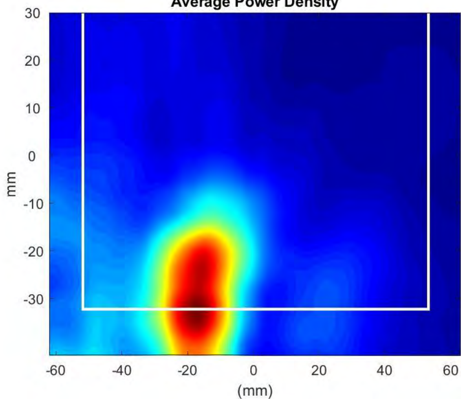
Phaser0 Beam Pair:29-157 Surface:S2 Average Power Density
