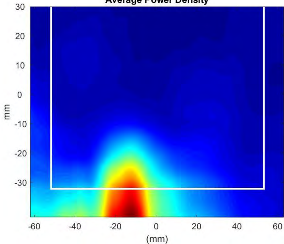
Phaser0 Beam Pair:43-169 Surface:S1 Average Power Density
