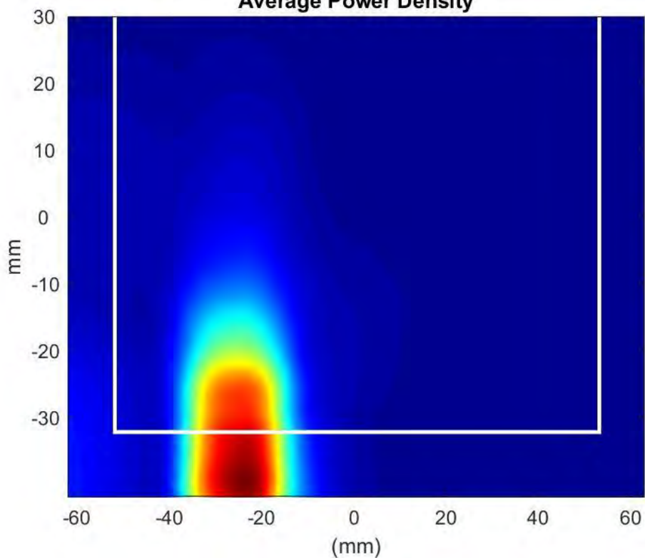
Phaser0 Beam Pair:45-171 Surface:S2 Average Power Density
