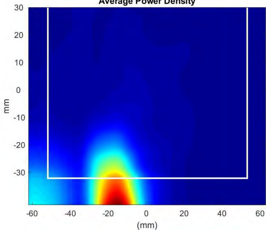
Phaser0 Beam Pair:55-183 Surface:S1 Average Power Density
