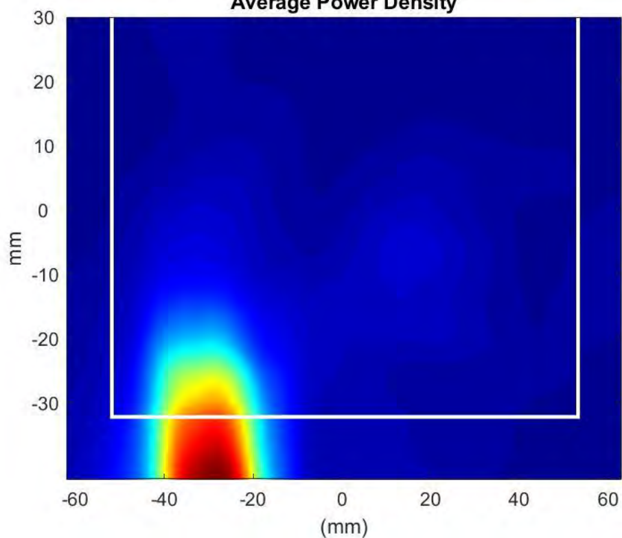
Phaser0 Beam Pair:56-185 Surface:S1 Average Power Density
