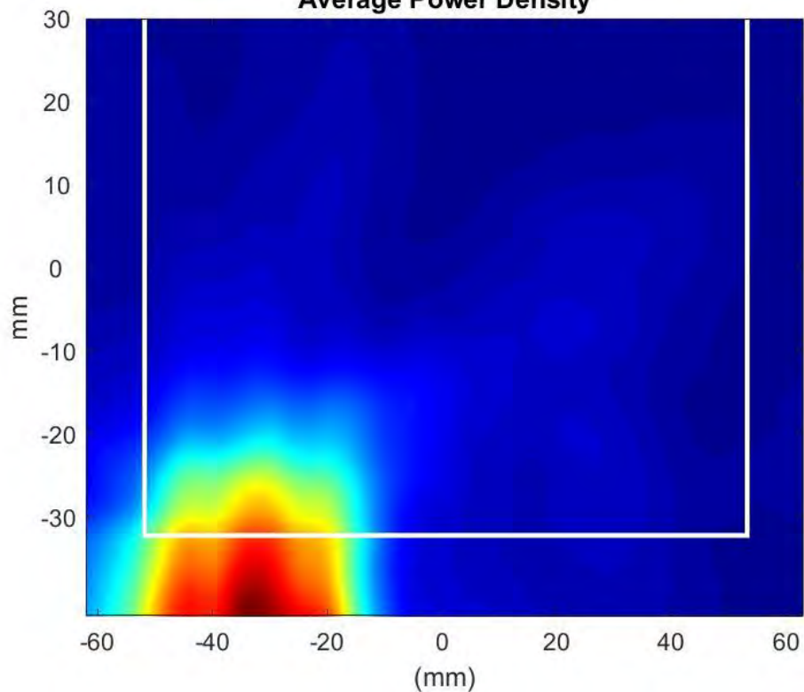
Phaser0 Beam Pair:16-144 Surface:S1 Average Power Density
