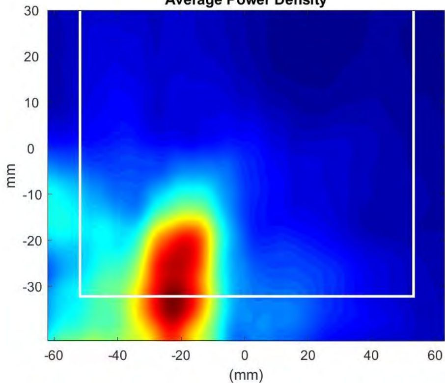
Phaser0 Beam Pair:14-141 Surface:S2 Average Power Density
