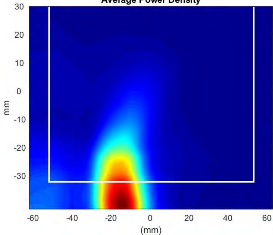
Phaser0 Beam Pair:55-183 Surface:S2 Average Power Density
