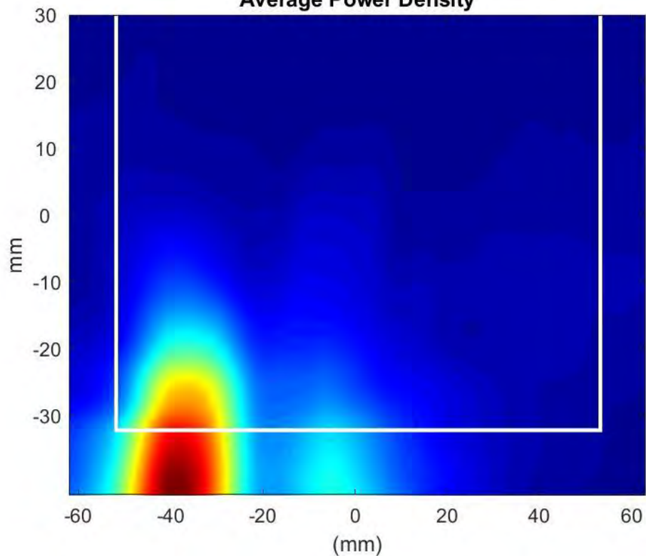
Phaser0 Beam Pair:41-172 Surface:S2 Average Power Density
