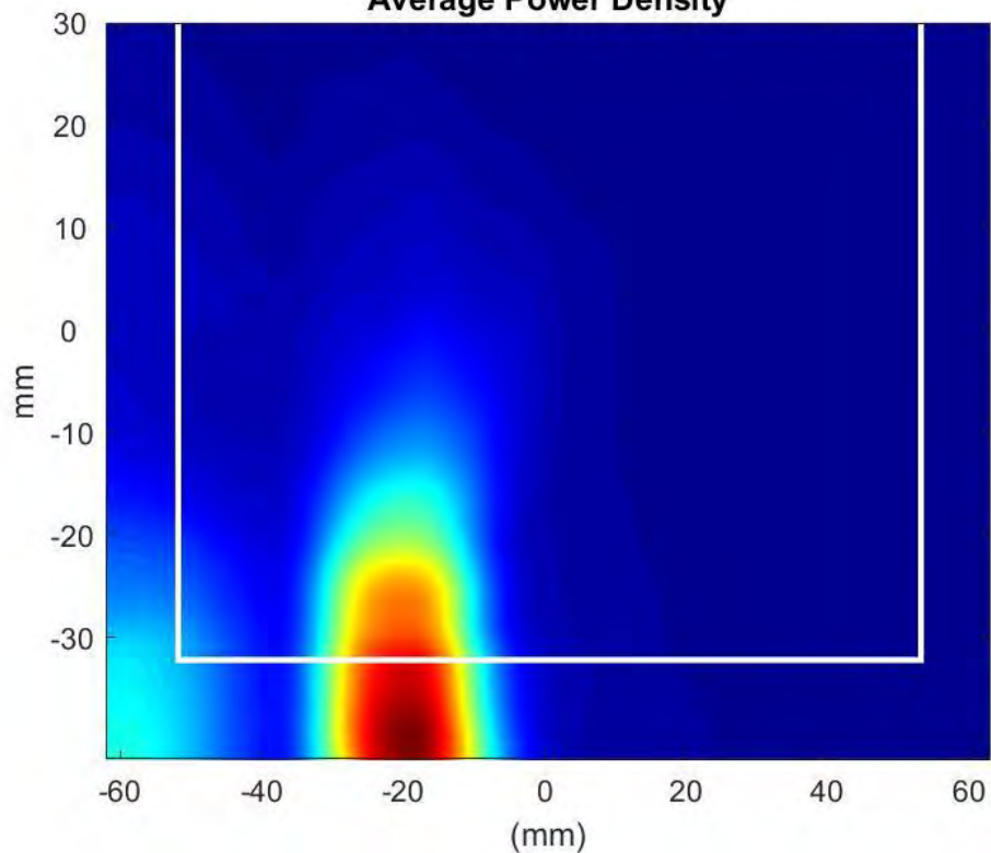
Phaser0 Beam Pair:30-158 Surface:S2 Average Power Density
