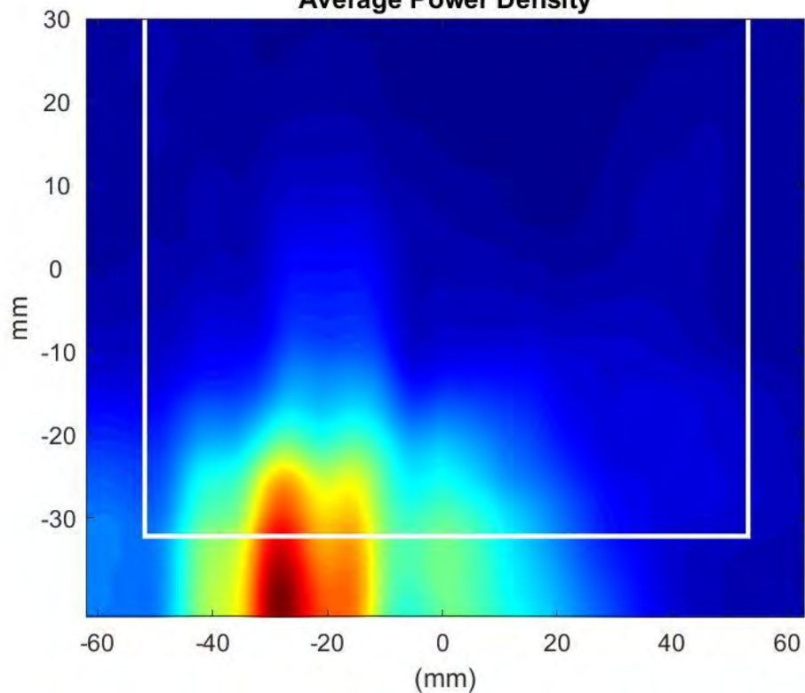
Phaser0 Beam Pair:3-131 Surface:S2 Average Power Density
