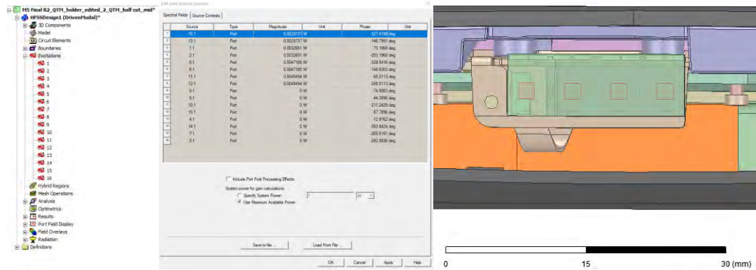
Figure 3-8 Antenna port excitations in ANSYS EM Suite 2019R2
