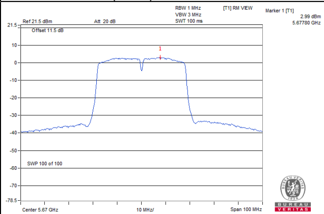
802.11n (HT40) / Chain 2 / CH 134
