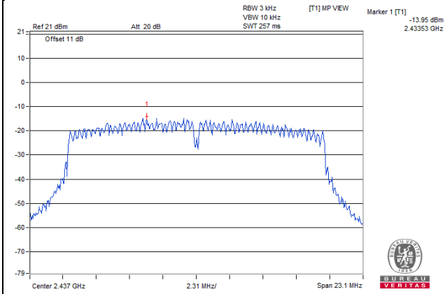
VHT20_Chain 1 / CH6
