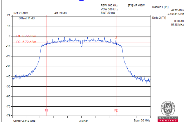
VHT20_Chain 1 / CH1
