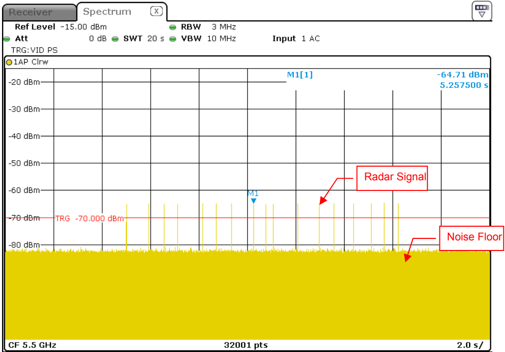
Radar Signal 5
