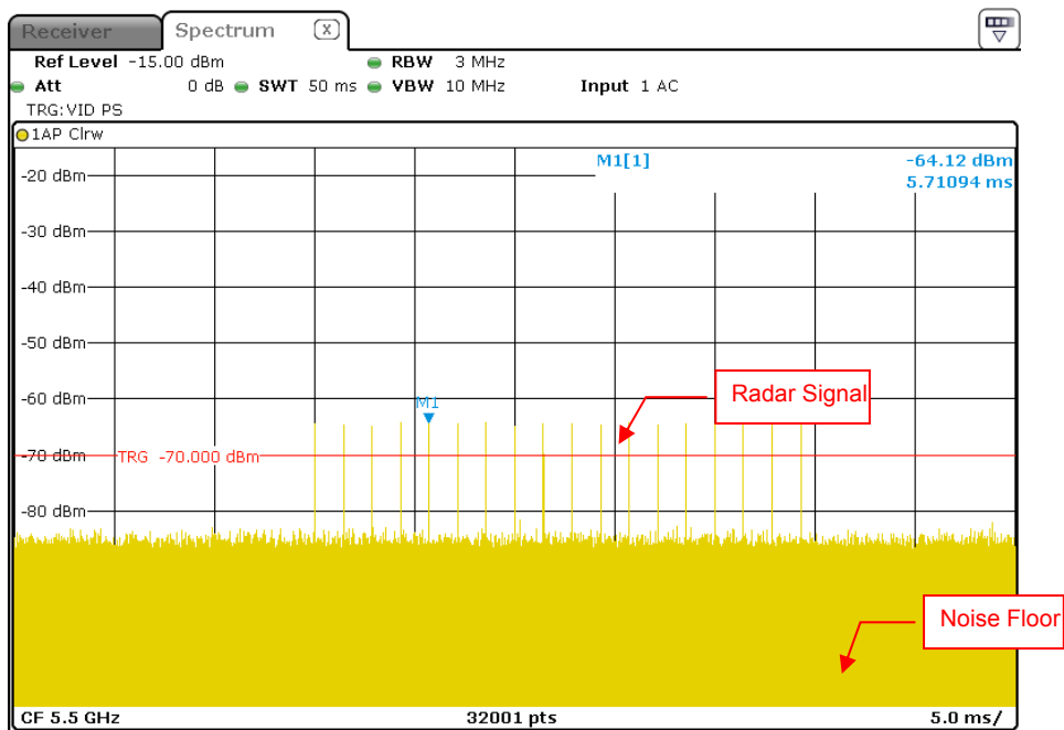
Radar Signal 0
