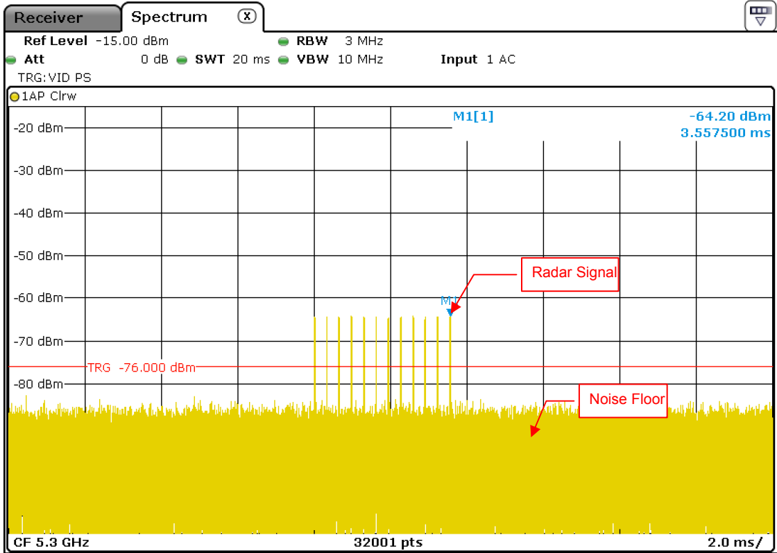
Radar Signal 4
