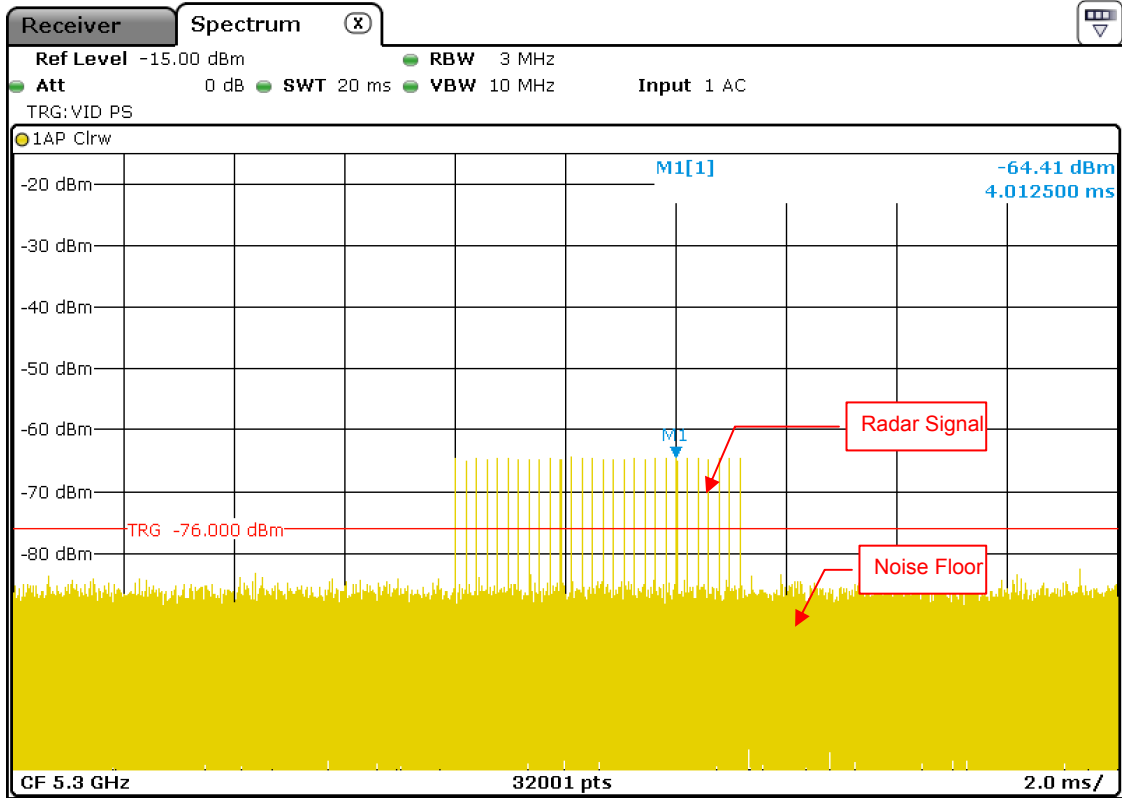
Radar Signal 2
