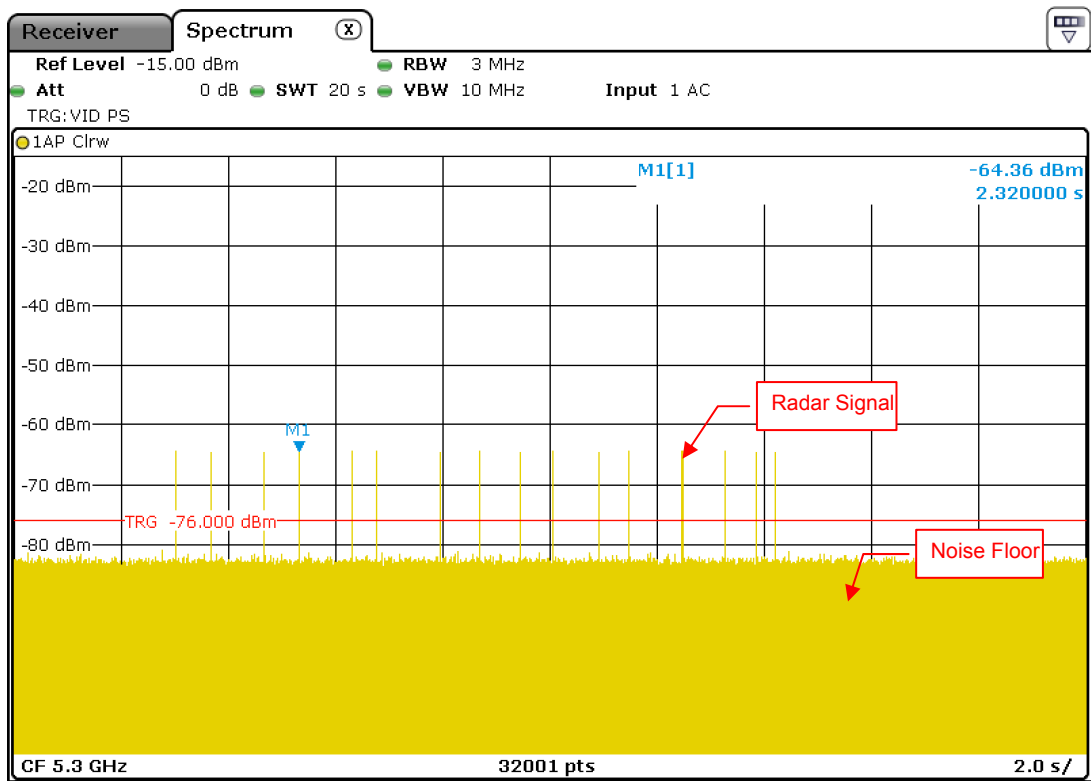
Radar Signal 5
