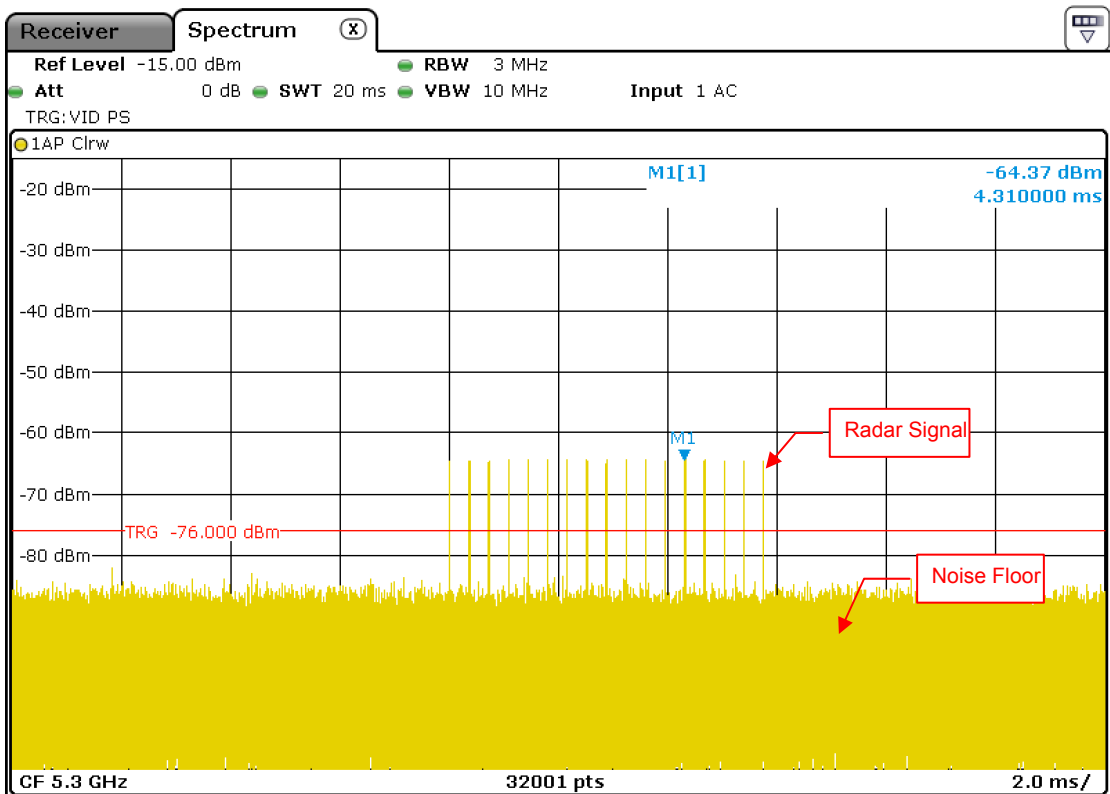
Radar Signal 3
