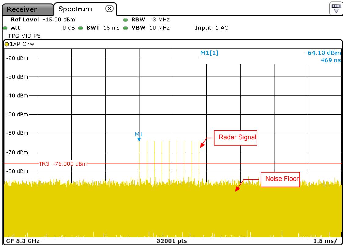
Radar Signal 6
