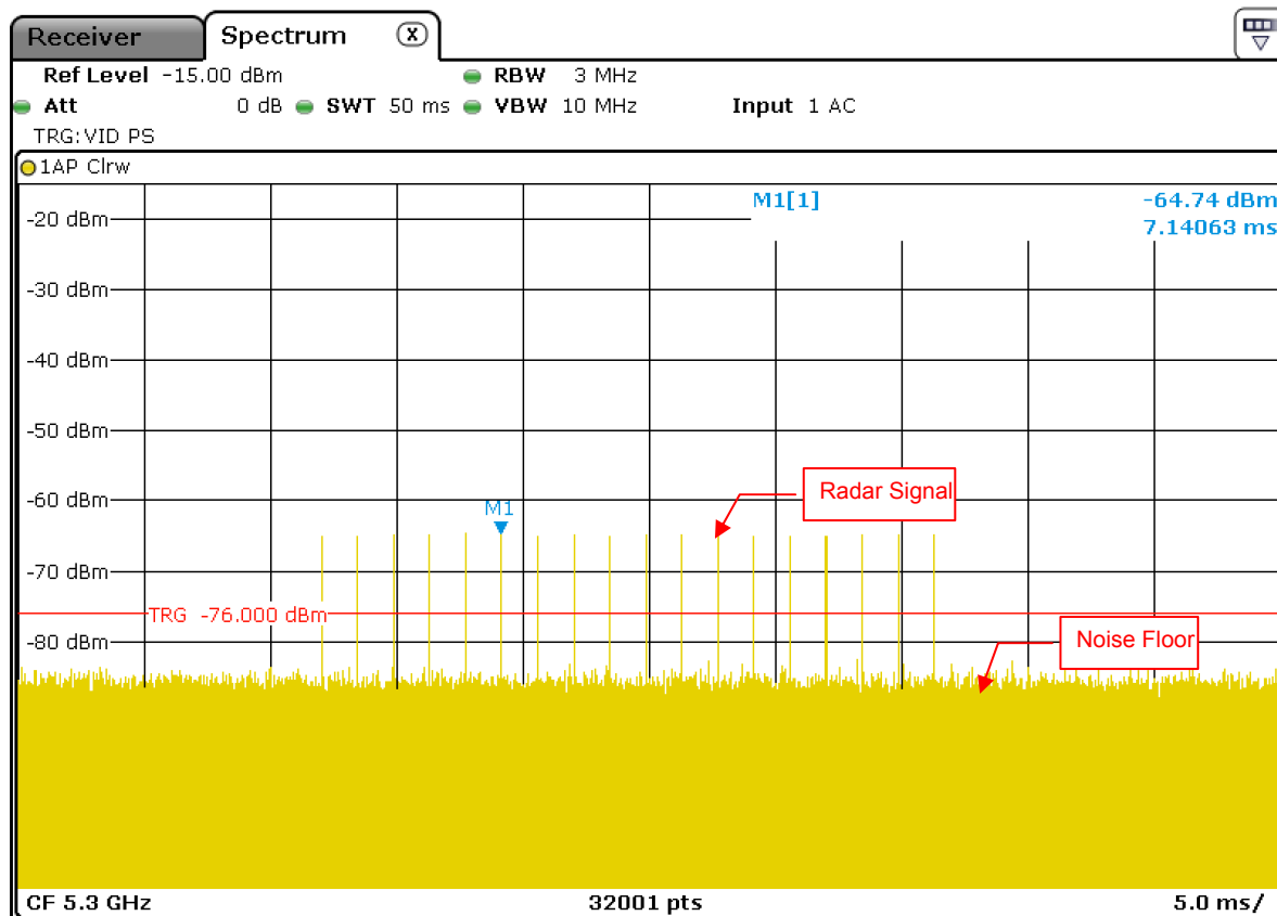
Radar Signal 0
