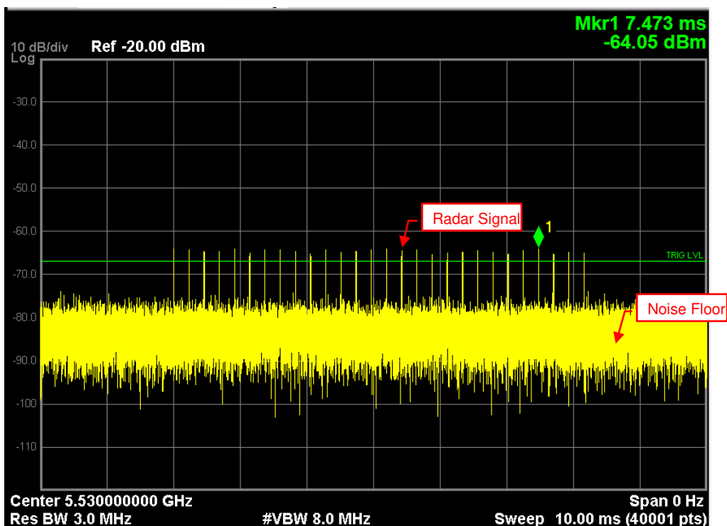
Radar Signal 2
