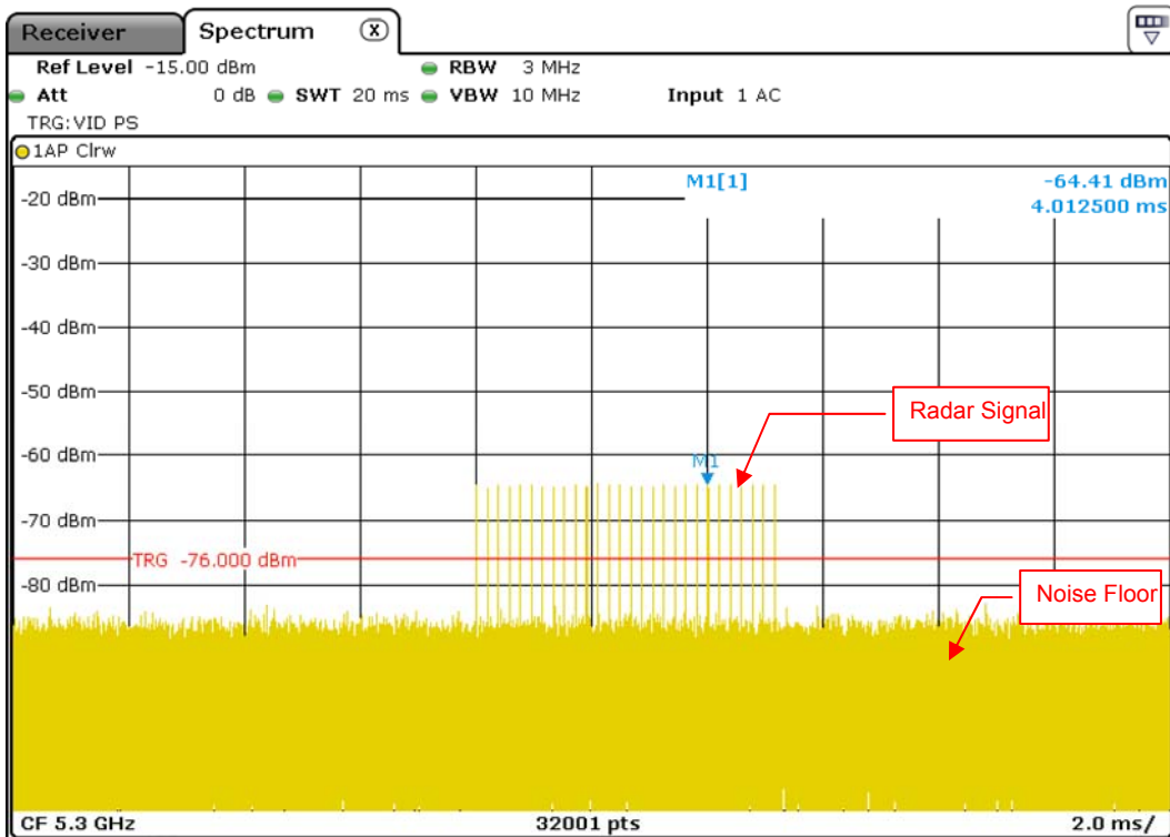
Radar Signal 2
