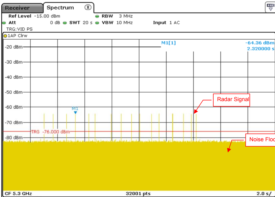
Radar Signal 5
