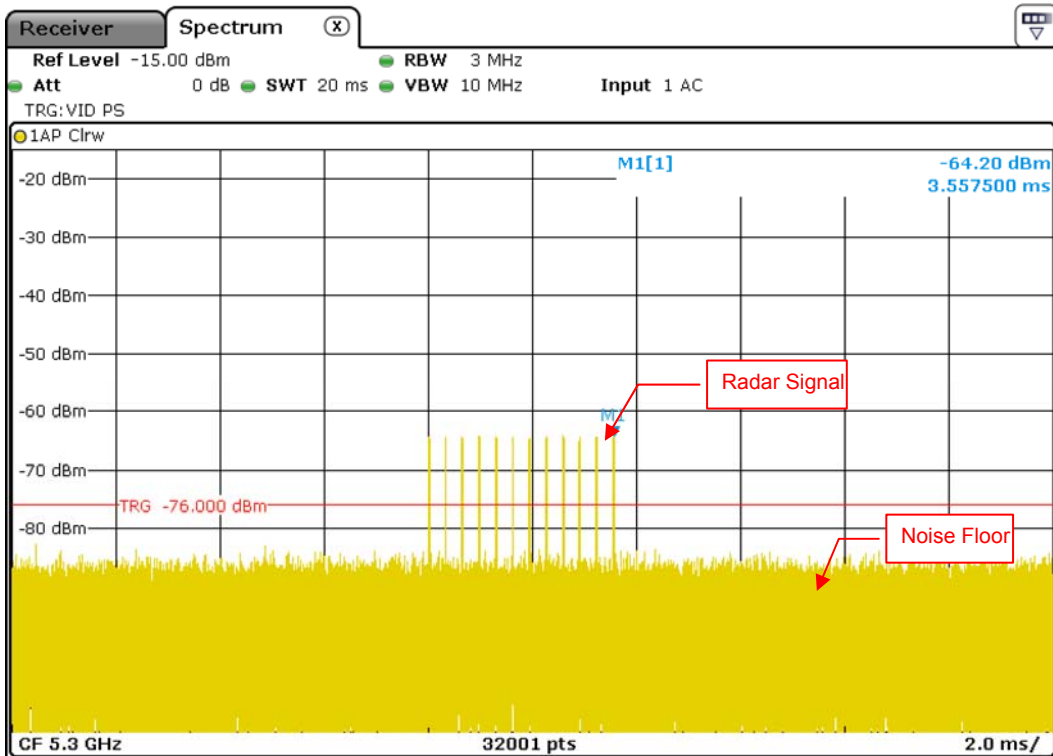
Radar Signal 4
