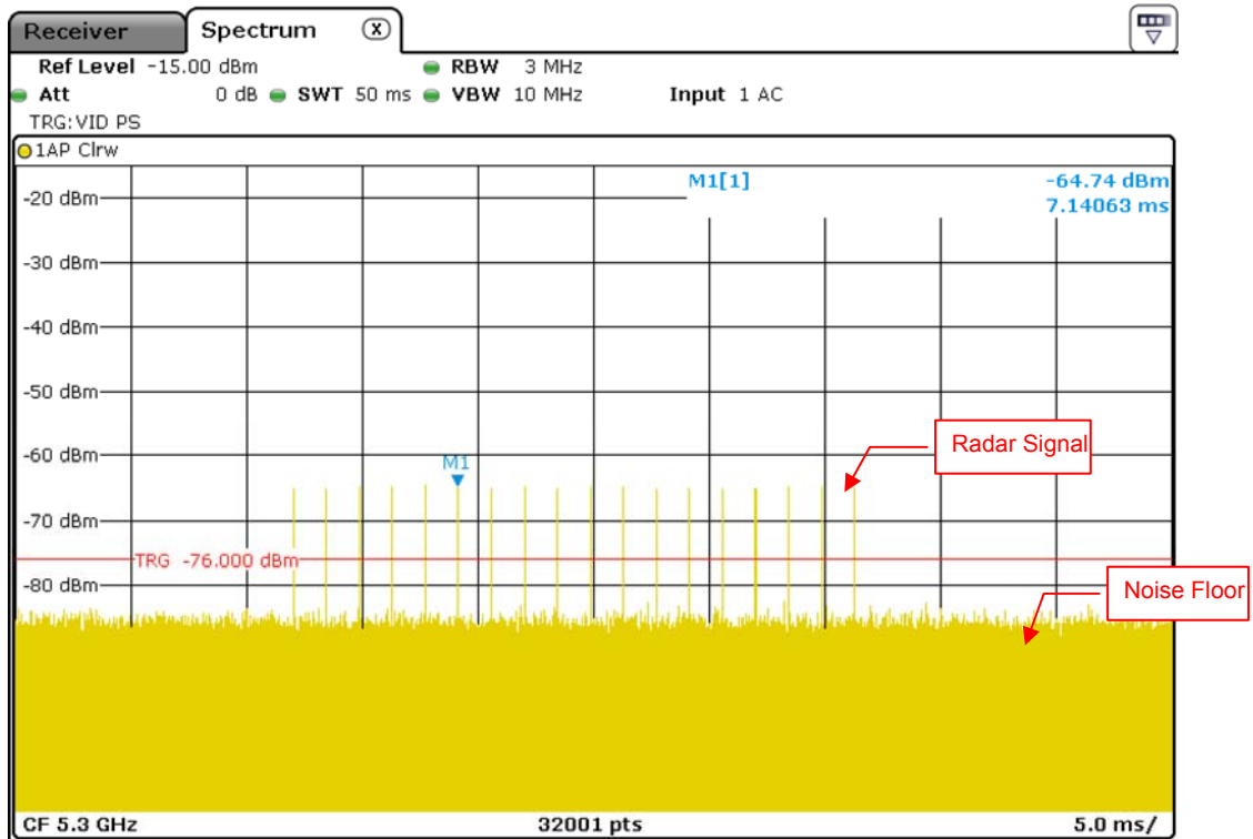
Radar Signal 0
