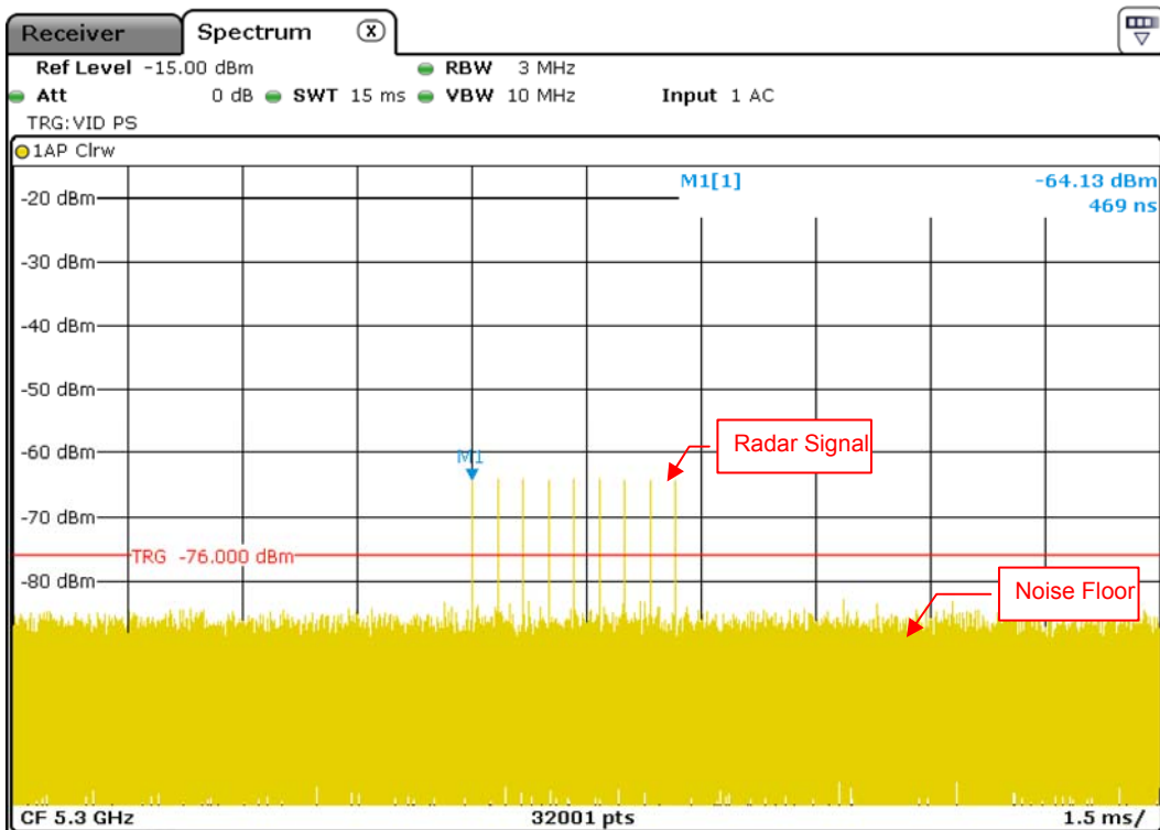
Radar Signal 6
