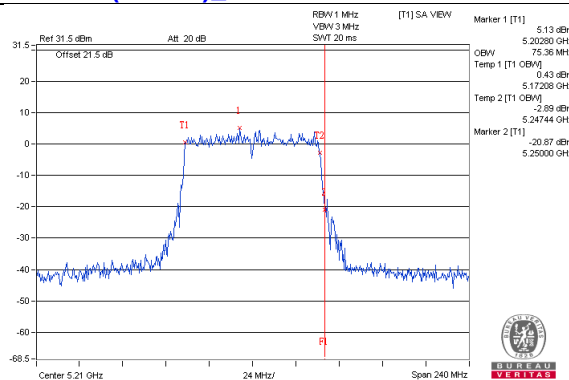
802.11ac(VHT80)_Chain1 / CH42
