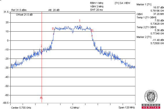
802.11ac(VHT40)_Chain1 / CH151
