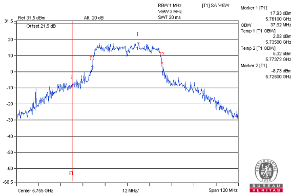
802.11ac(VHT40)_Chain2 / CH151
