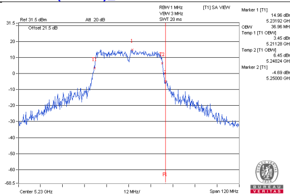
802.11ac(VHT40)_Chain1 / CH46
