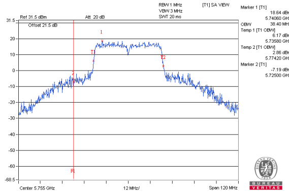
802.11ac(VHT40)_Chain1 / CH151
