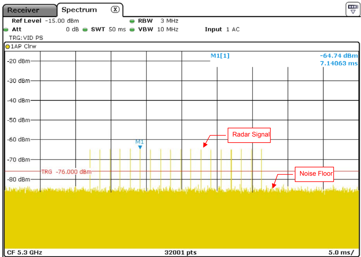
Radar Signal 0
