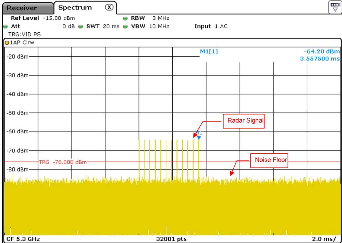
Radar Signal 4
