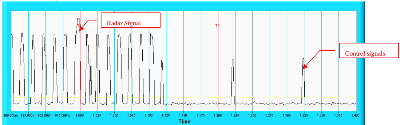
Channel Closing Transmission Time & Channel Move Time
