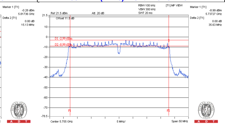
802.11n (HT40) – Chain 0: CH 151
