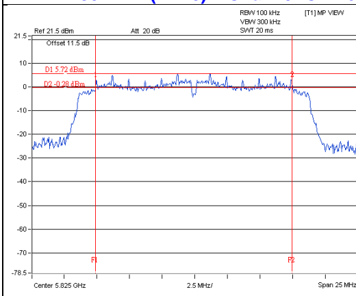
802.11n (HT20) – Chain 0: CH 165
