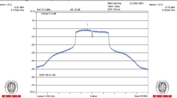
802.11n (HT20) / Ch 157 / chain 2
