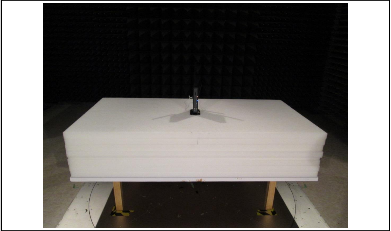
Radiated Emission Test (POE Mode)
