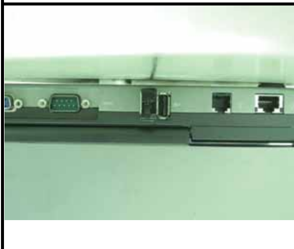
VERTICAL FRONT WITH 0.5 CM GAP
