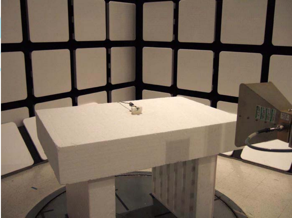
Test Configuration 2: 960 MHz – 40 GHz
