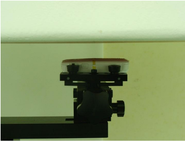
Front of the DUT with Phantom 2 cm Gap
