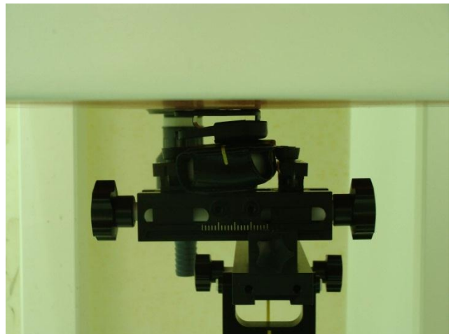
Back of the DUT with Phantom 0 cm Gap (with Holster)
