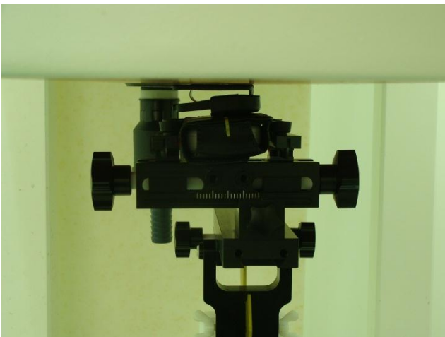
Front of the DUT with Phantom 0 cm Gap (with Holster)
