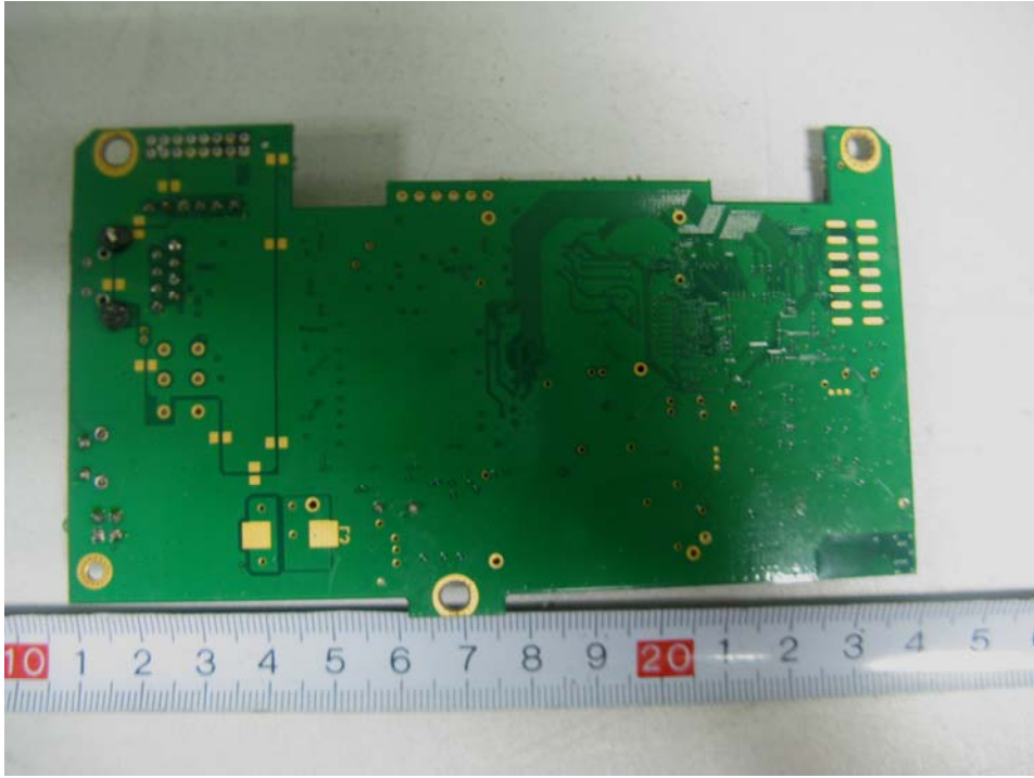
EUT – Main Board Bottom Components View
