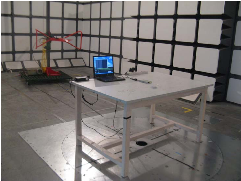
30-1000MHz: Radiated Emissions - Front View (Antenna 2)
