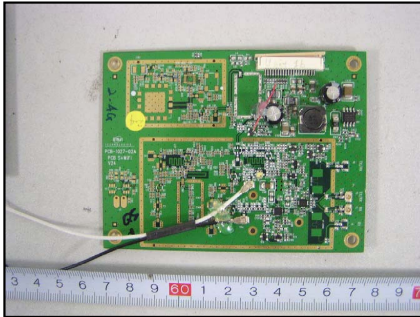
EUT – RF Board Top View
