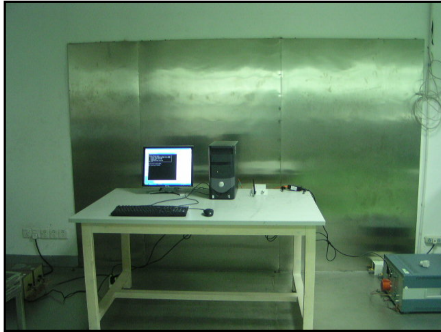
Conducted Emissions - Front View
