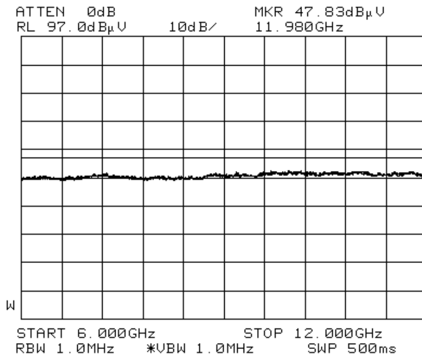
Channel 1 @ 802.11g 54Mbps (6GHz-12GHz)
