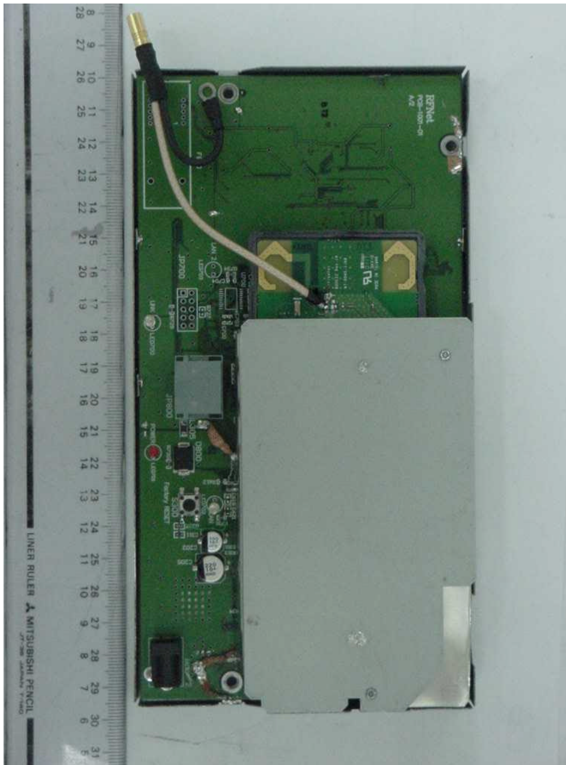
EUT Internal View – Top View Without Bottom Casing
