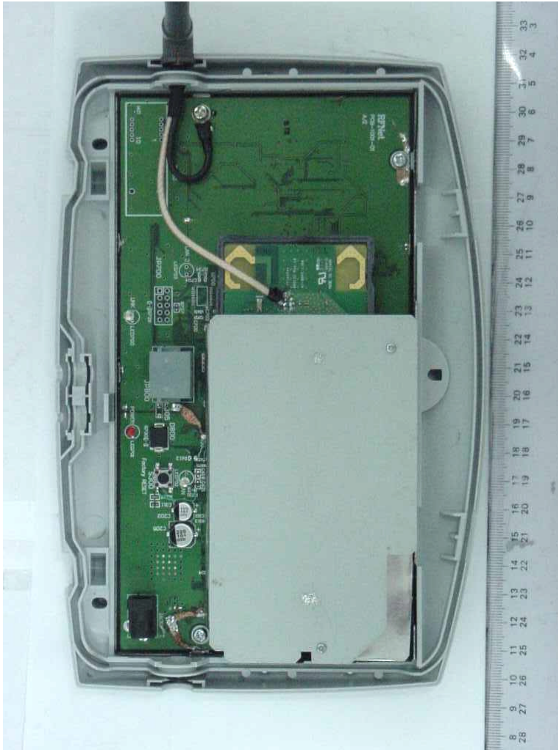
EUT Internal View – Top View With Bottom Casing
