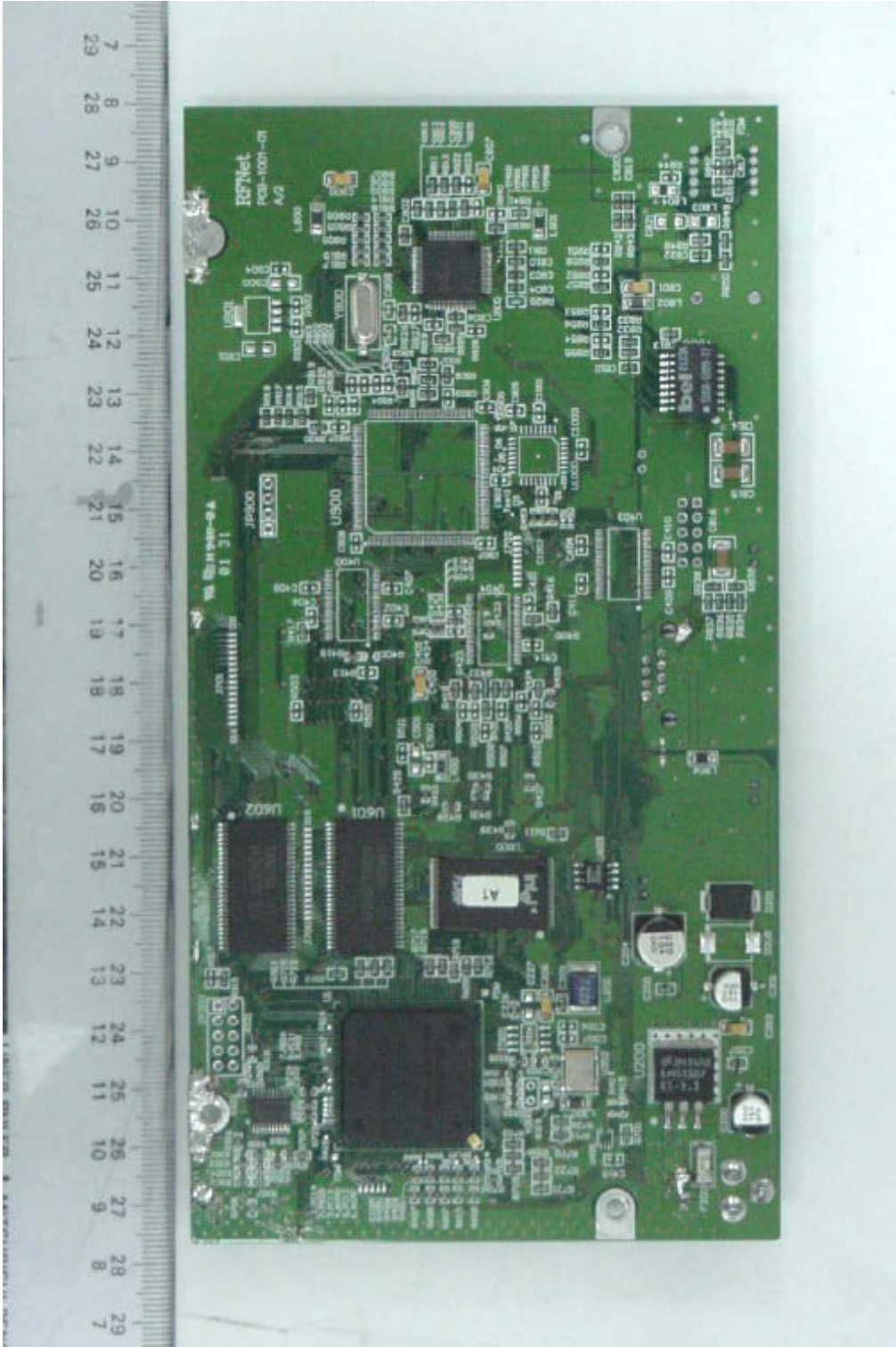
EUT Mother Board – Bottom View With Shield Removed
