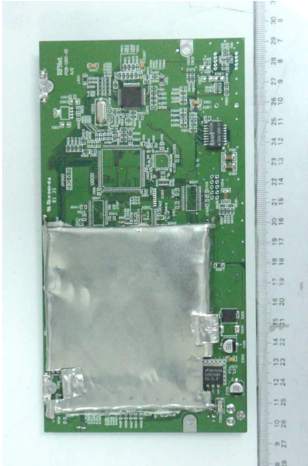
EUT Mother Board – Bottom View With Shield
