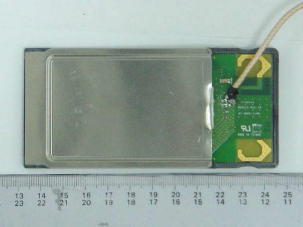
Daughter Board – Top View
