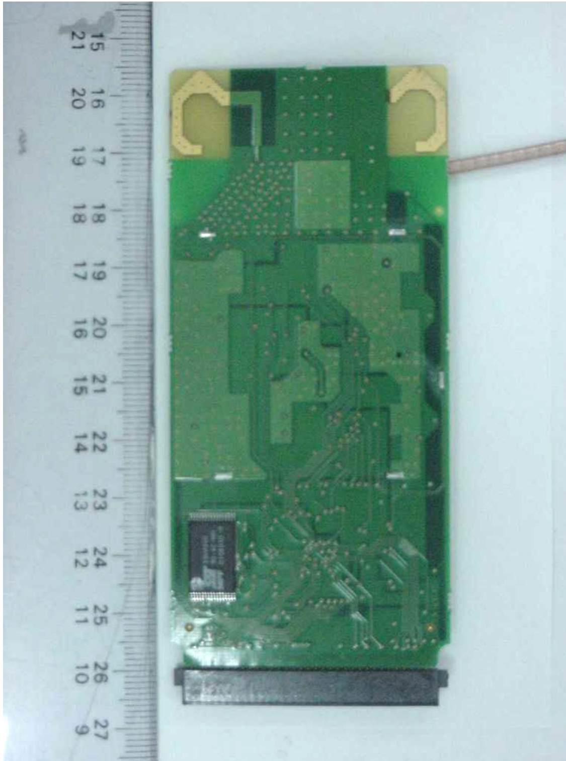
Daughter Board – Bottom View With Shield Removed
