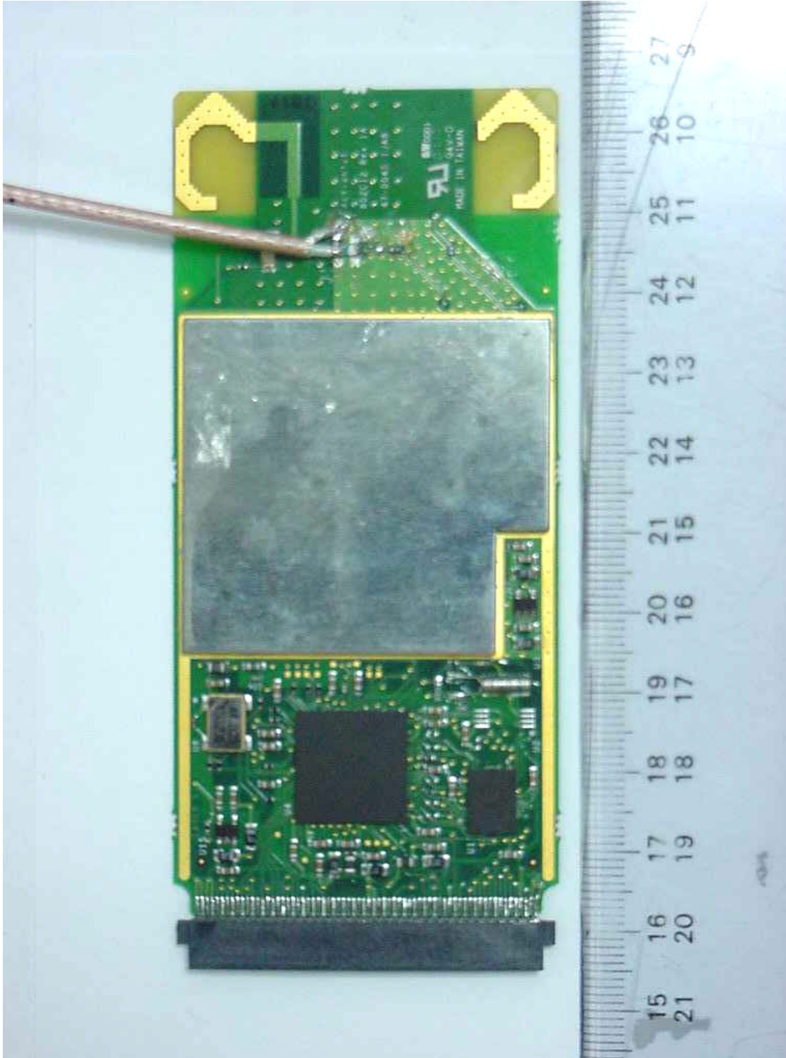
Daughter Board – Top View With Shield Removed
