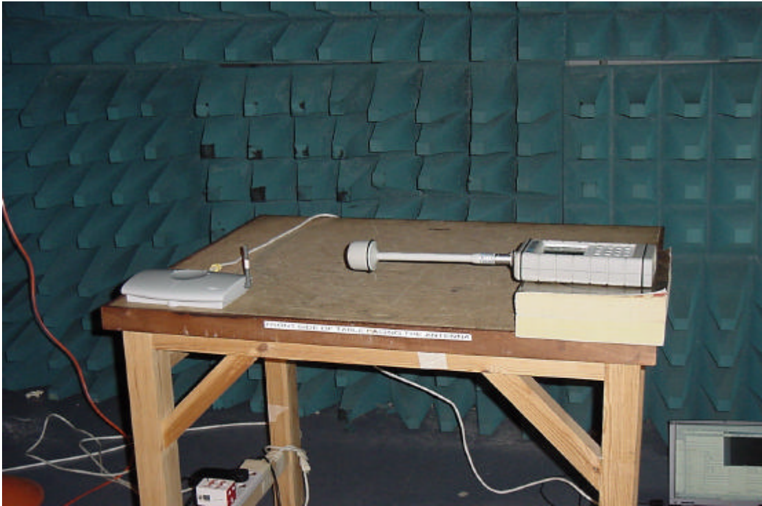
Maximum Permissible Exposure Measurements – General View
