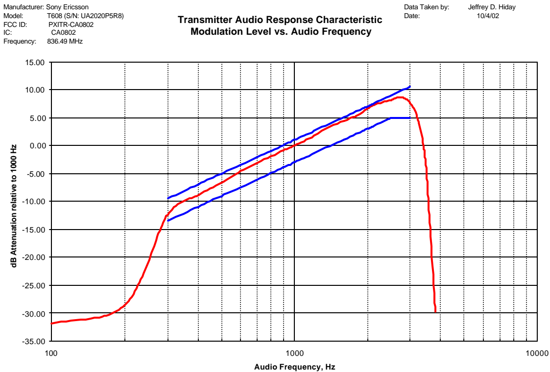
Figure 6-1: Audio Filter Characteristics
