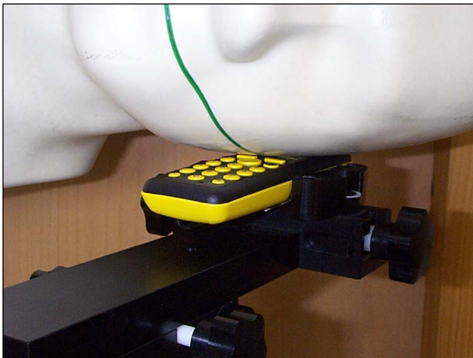
EUT Left Ear Tilted
