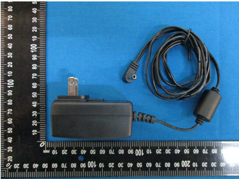
Host - AC/DC Adaptor
