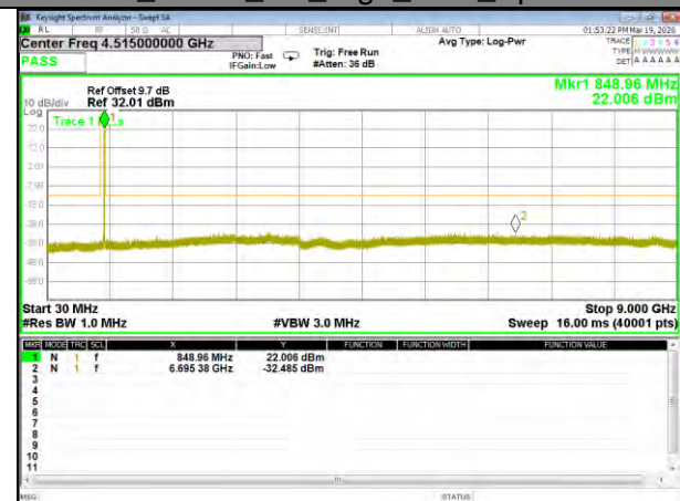
B26_QPSK_3M_High_CDT_Spurious
