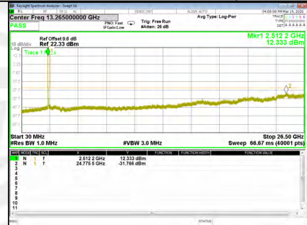
B41_Q16_20M_Low_CDT_Spurious
