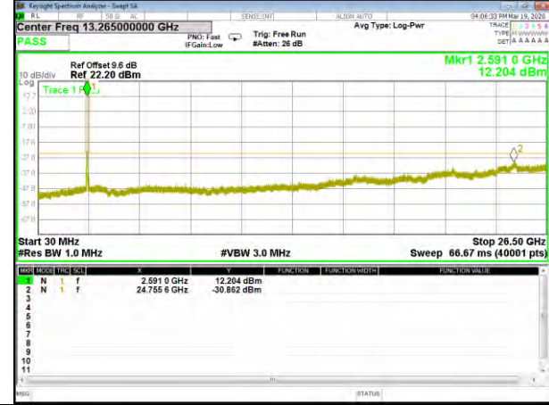
B41_Q16_20M_Mid_CDT_Spurious
