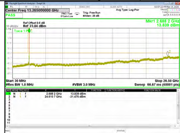
B41_Q16_15M_Low_CDT_Spurious
