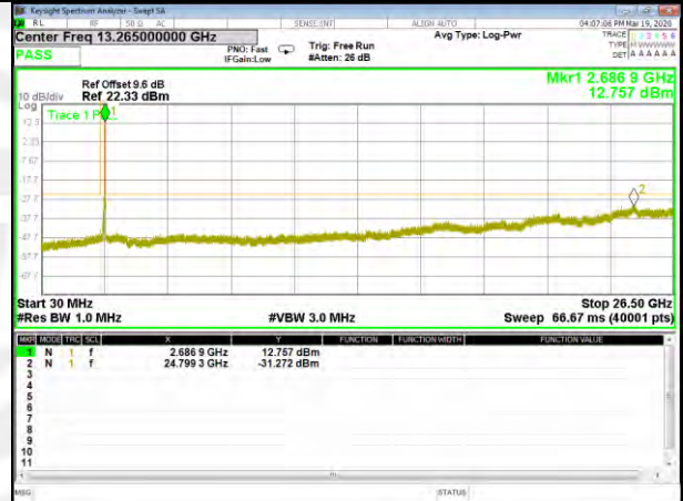
B41_Q16_20M_High_CDT_Spurious
