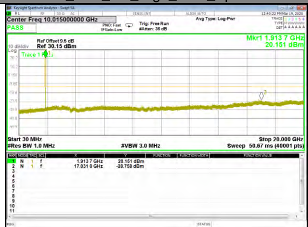
B25_Q16_3M_High_CDT_Spurious
