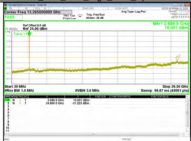
B41_Q16_10M_High_CDT_Spurious
