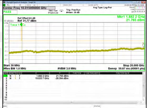
B25_Q16_1.4M_High_CDT_Spurious
