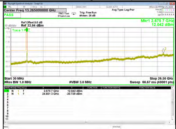
B41_Q16_20M_High_CDT_Spurious
