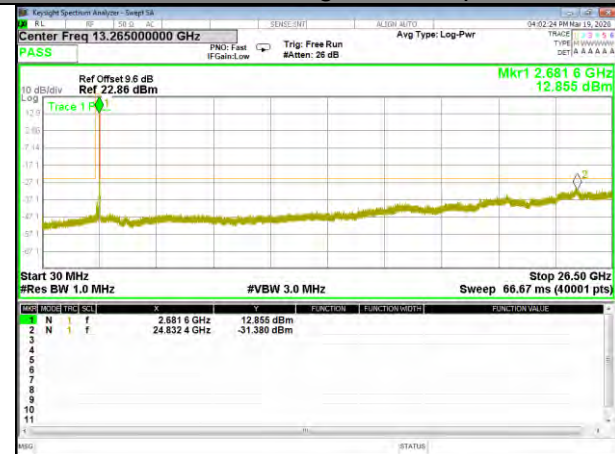
B41_Q16_15M_High_CDT_Spurious
