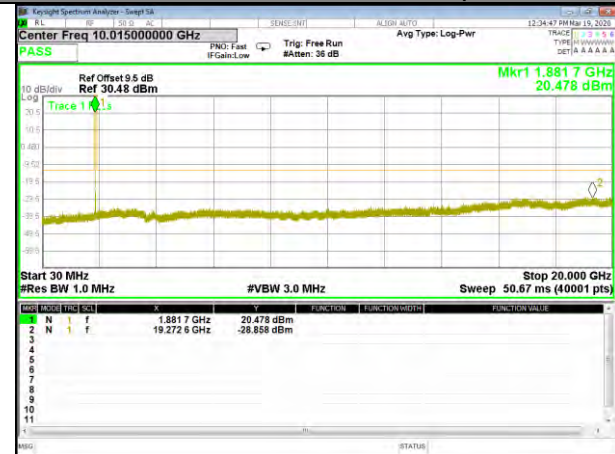
B25_QPSK_3M_High_CDT_Spurious
