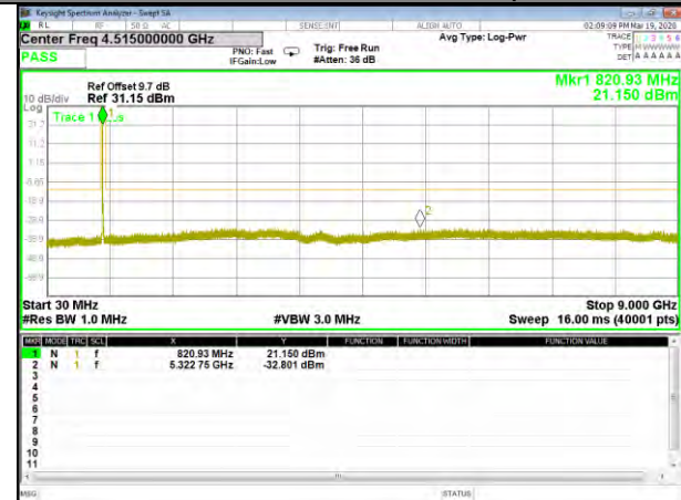
B26_QPSK_5M_High_CDT_Spurious
