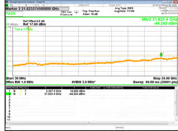
B30_QPSK_5M_Mid_CDT_Spurious
