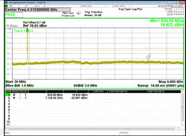
B26_Q16_10M_Mid_CDT_Spurious
