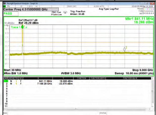
B26_Q16_15M_High_CDT_Spurious
