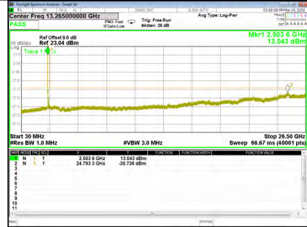
B41_QPSK_15M_High_CDT_Spurious
