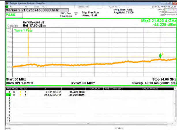
B30_QPSK_5M_High_CDT_Spurious
