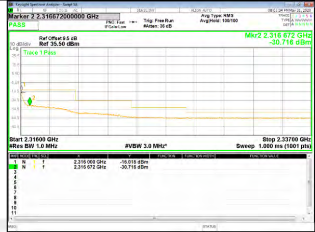
B30_16QAM_5M_Low_1-RB_Bedge
