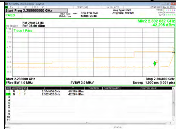
B30_16QAM_5M_Low_full-RB_Bedge
