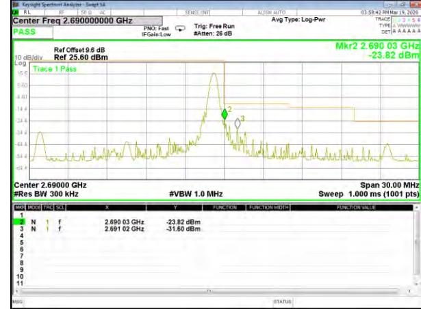
B41_QPSK_15M_High_Full-RB_Bedge
