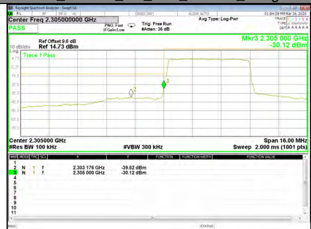
B30_16QAM_5M_Low_Full-RB_Bedge
