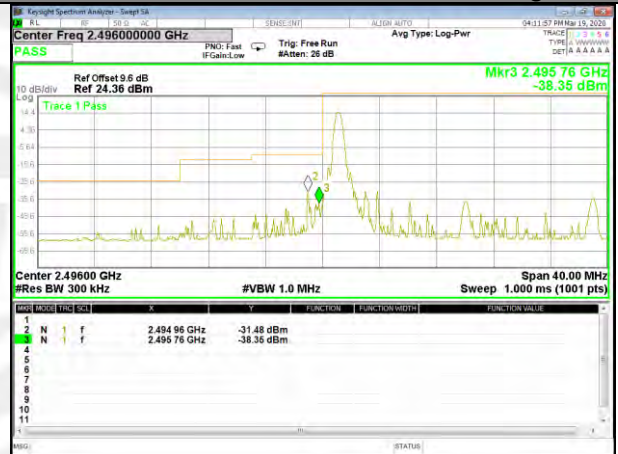
B41_16QAM_20M_Low_Full-RB_Bedge
