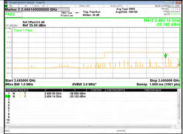
B41_QPSK_20M_Low_full-RB_Bedge
