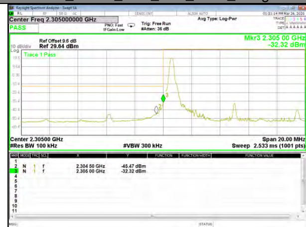
B30_QPSK_10M_Low_1-RB_Bedge
