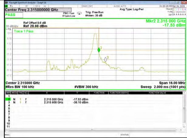
B30_16QAM_5M_High_Full-RB_Bedge
