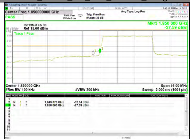
B25_QPSK_5M_Low_Full-RB_Bedge
