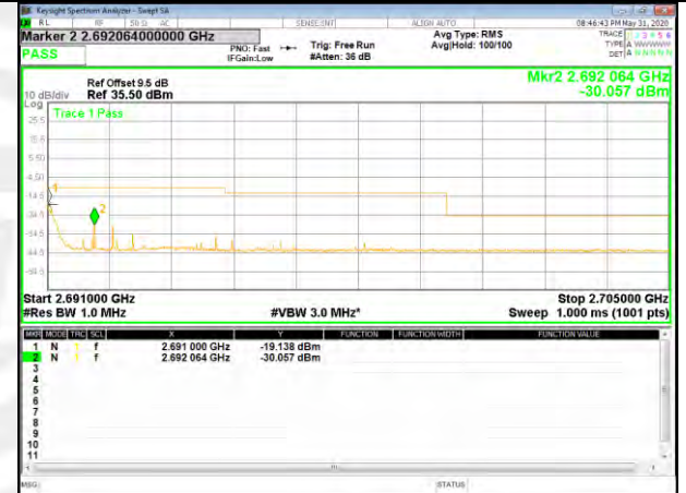
B41_QPSK_10M_High_full-RB_Bedge
