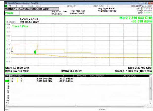
B30_QPSK_10M_High_full-RB_Bedge
