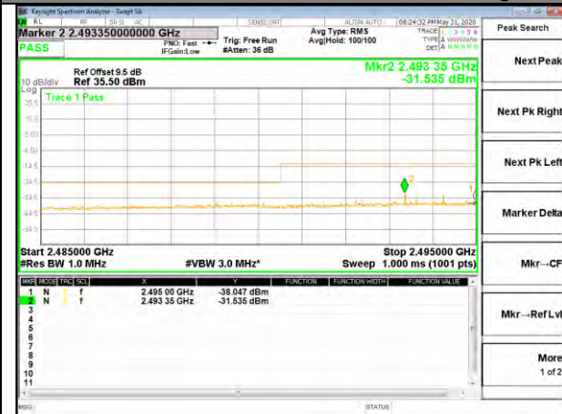
B41_16QAM_20M_Low_full-RB_Bedge
