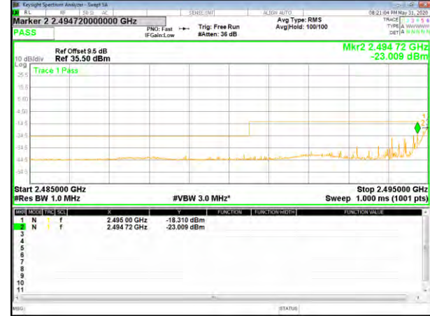
B41_16QAM_10M_Low_full-RB_Bedge
