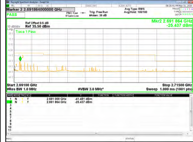
B41_16QAM_20M_High_full-RB_Bedge
