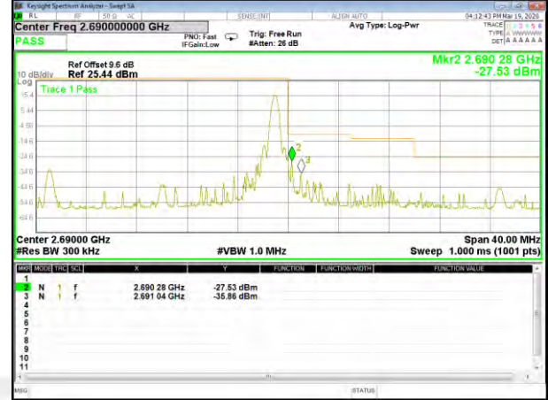
B41_16QAM_20M_High_Full-RB_Bedge
