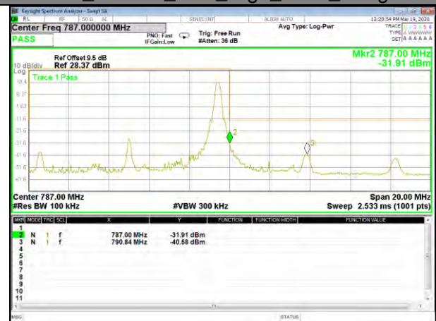
B13_16QAM_10M_High_1-RB_Bedge
