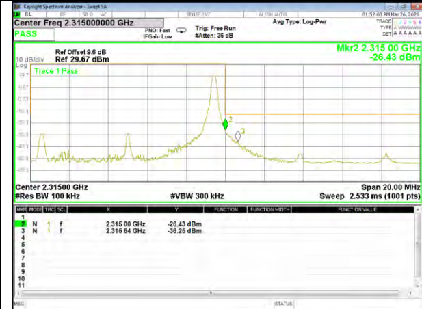
B30_QPSK_10M_High_Full-RB_Bedge
