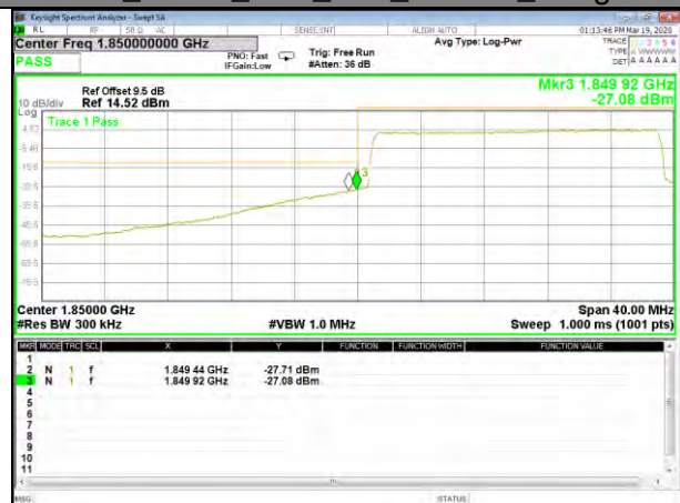
B25_QPSK_20M_Low_Full-RB_Bedge
