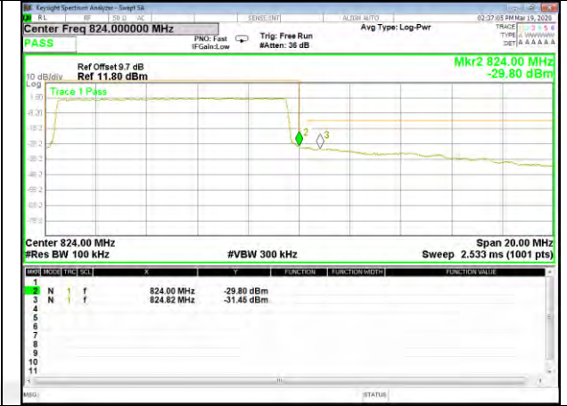
B26_Q16_10M_High_Full-RB_Bedge
