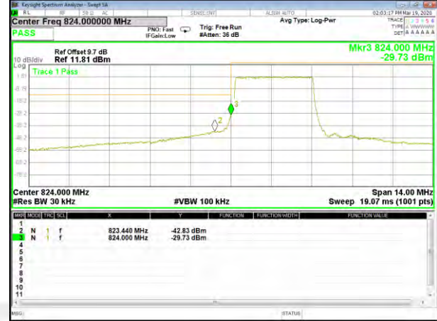
B26_Q16_3M_High_Full-RB_Bedge
