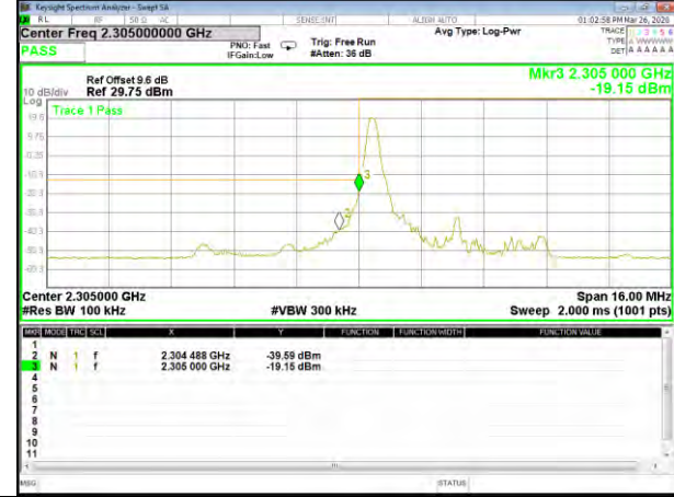
B30_QPSK_5M_Low_Full-RB_Bedge
