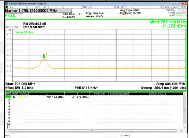
B13_QPSK_10M_High_full-RB_Bedge
