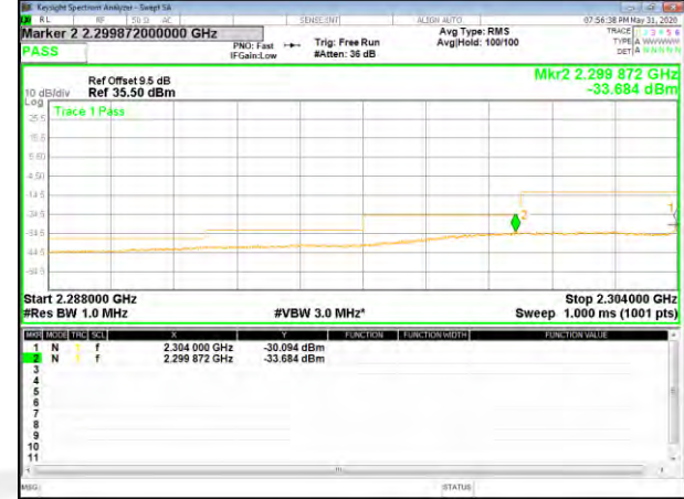
B30_QPSK_10M_High_1-RB_Bedge
