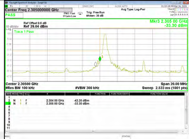
B30_16QAM_10M_Low_Full-RB_Bedge
