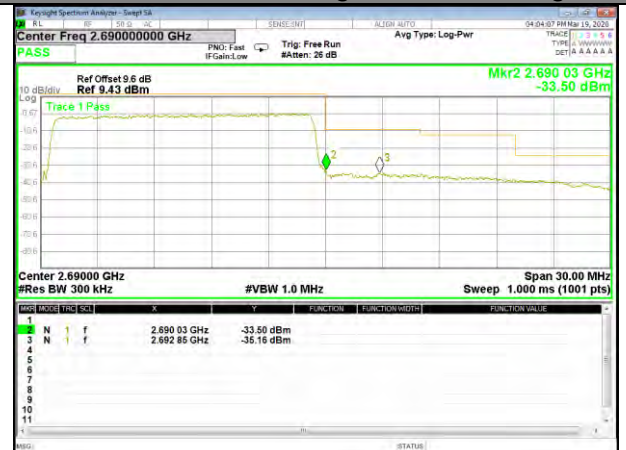
B41_16QAM_15M_High_Full-RB_Bedge
