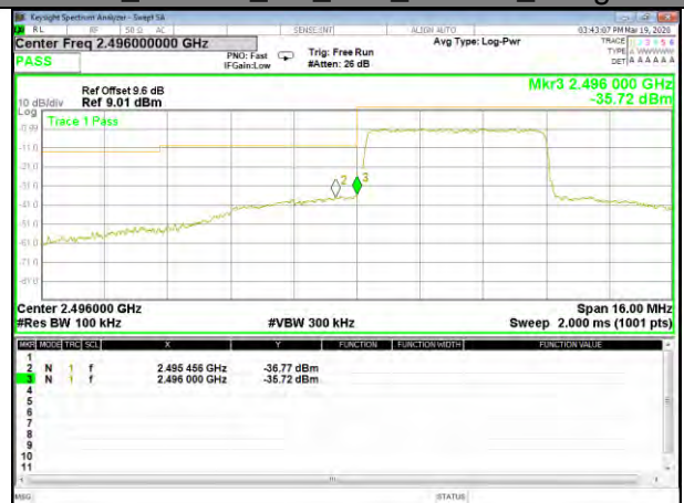
B41_16QAM_5M_Low_Full-RB_Bedge
