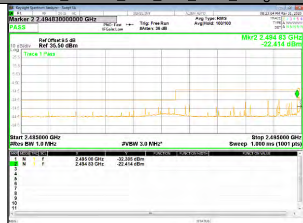
B41_16QAM_15M_Low_1-RB_Bedge
