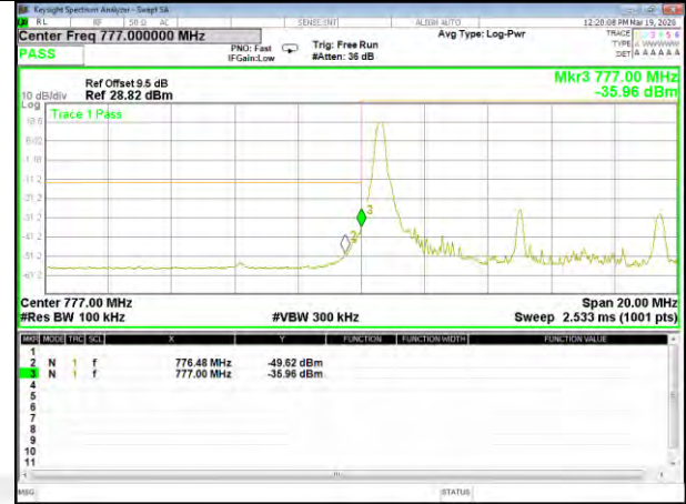
B13_16QAM_10M_Low_Full-RB_Bedge
