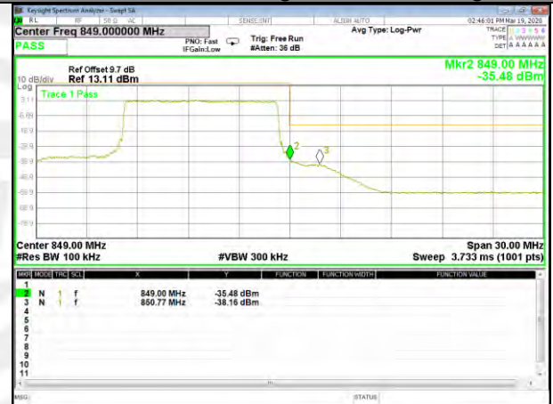
B26_Q16_15M_High_Full-RB_Bedge
