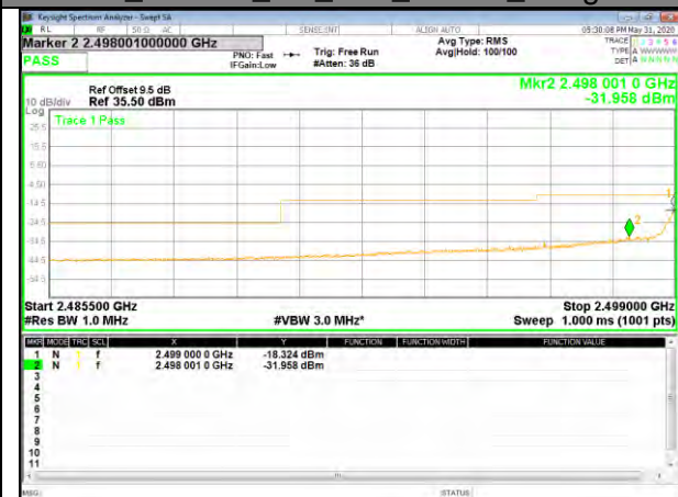
B7_16QAM_5M_Low_full-RB_Bedge
