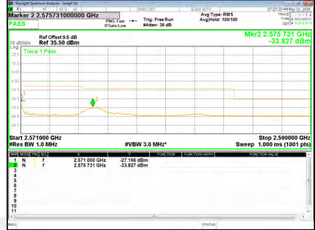
B7_QPSK_15M_High_full-RB_Bedge
