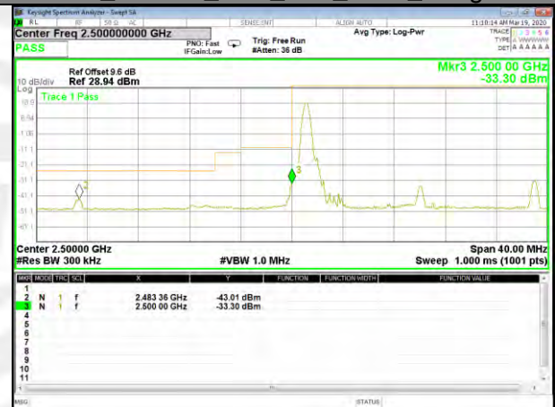
B7_16QAM_20M_Low_Full-RB_Bedge
