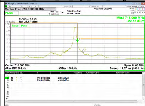
B12_QPSK_3M_High_1-RB_Bedge
