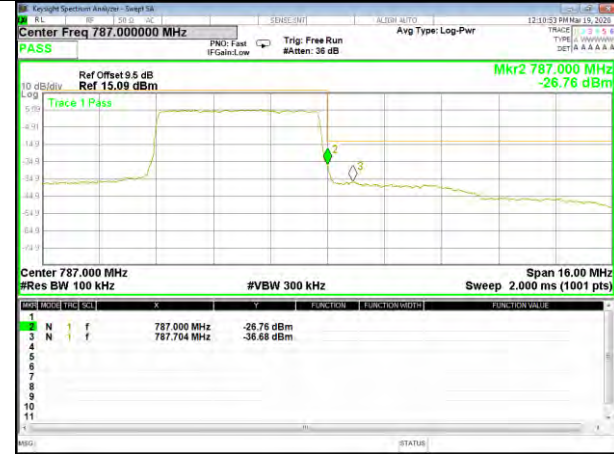
B13_16QAM_5M_Low_1-RB_Bedge
