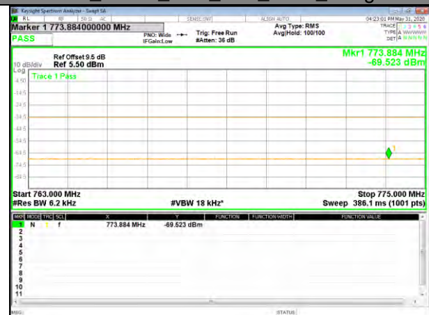
B13_QPSK_10M_Low_1-RB_Bedge
