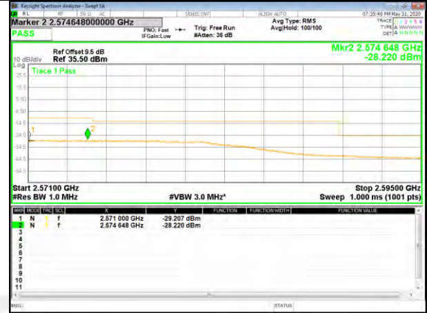
B7_16QAM_20M_Low_1-RB_Bedge
