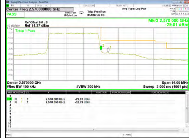
B7_16QAM_5M_Low_1-RB_Bedge
