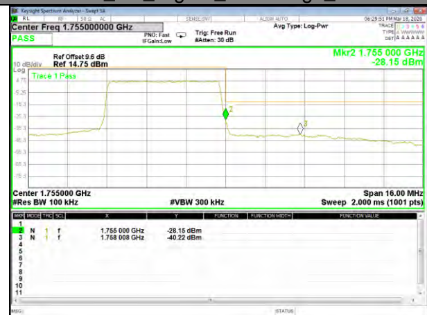
16QAM_5M_Higher_Band edge_Full-RB
