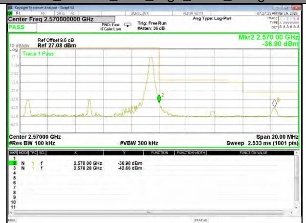
B7_16QAM_10M_High_1-RB_Bedge
