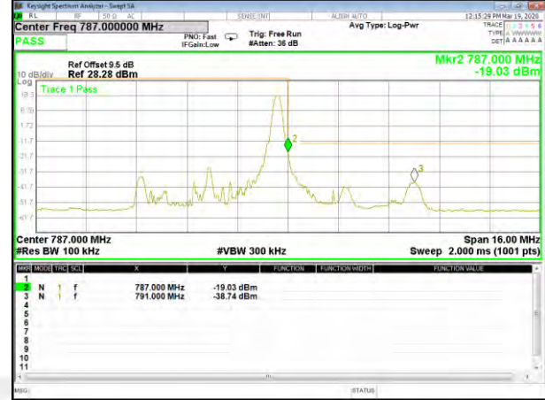
B13_16QAM_5M_High_Full-RB_Bedge
