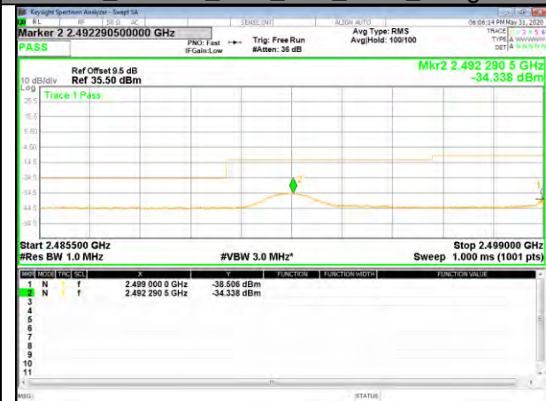
B7_16QAM_20M_Low_full-RB_Bedge
