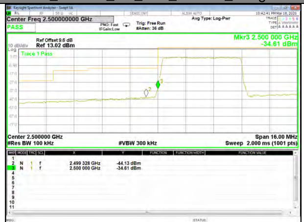
B7_16QAM_5M_Low_Full-RB_Bedge
