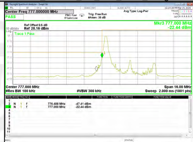
B13_16QAM_5M_Low_Full-RB_Bedge
