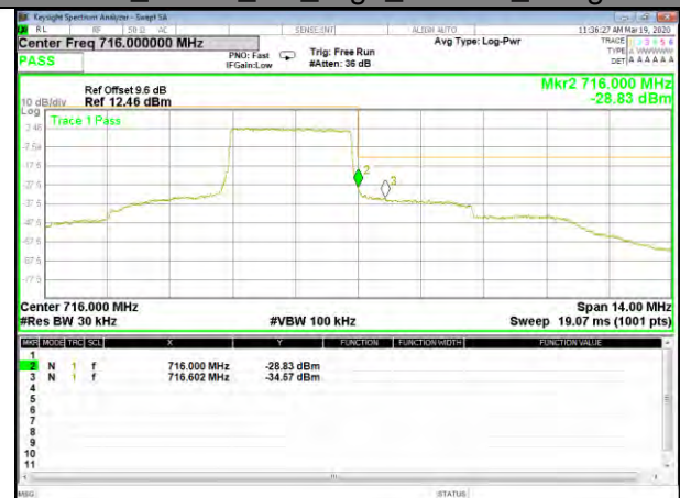
B12_QPSK_3M_High_Full-RB_Bedge
