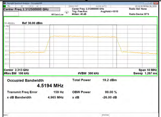
B30_Q16_5M_High_26BW-99%
