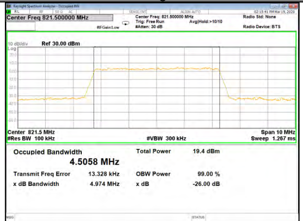
B26_Q16_5M_High_26BW-99%
