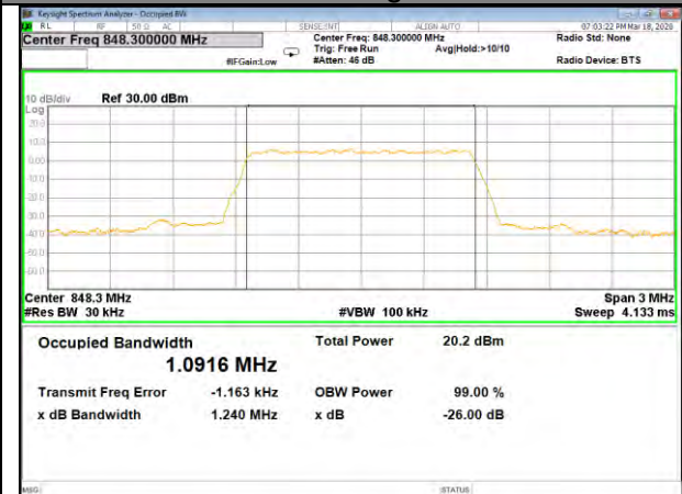
B5_QPSK_1.4M_High_26BW-99%
