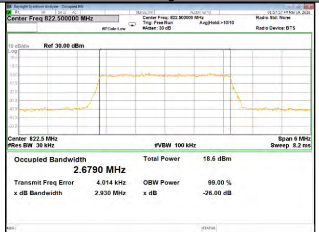
B26_Q16_3M_High_26BW-99%
