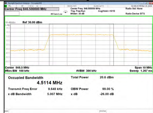
B26_QPSK_5M_High_26BW-99%
