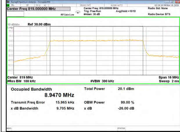
B26_QPSK_10M_Mid_26BW-99%
