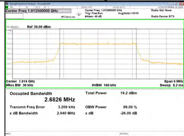
B25_QPSK_3M_High_26BW-99%
