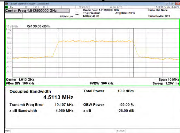
B25_QPSK_5M_High_26BW-99%
