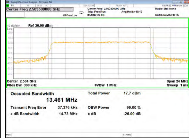
B41_QPSK_15M_High_26BW-99%
