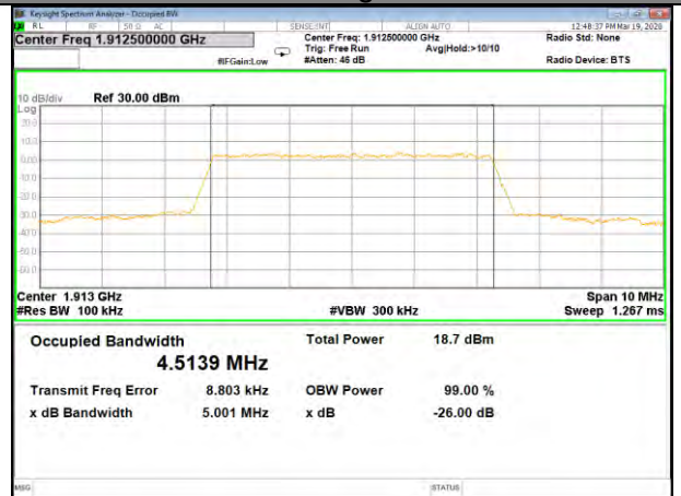
B25_Q16_5M_High_26BW-99%
