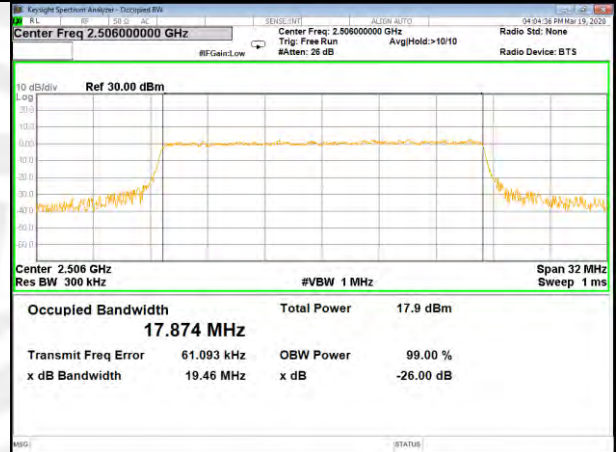
B41_Q16_20M_Low_26BW-99%
