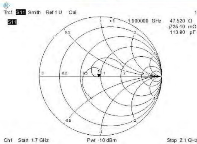
Impedance
