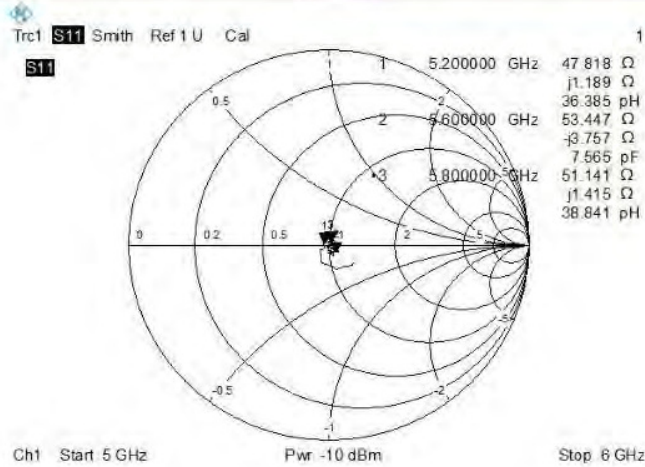
Impedance
