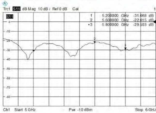
Return Loss
