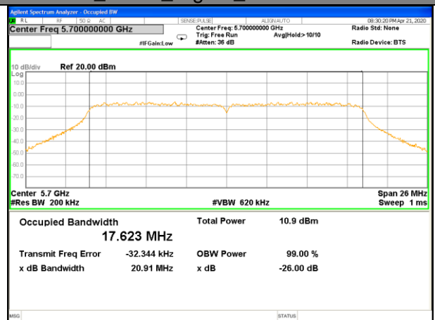
W56_11n20_Higher_26BW and 99%
