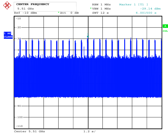
EUT Client Data Traffic Plot
