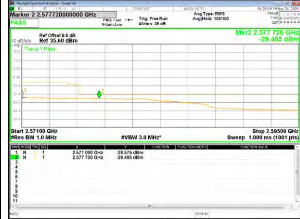
B7_16QAM_20M_Low_1-RB_Bedge
