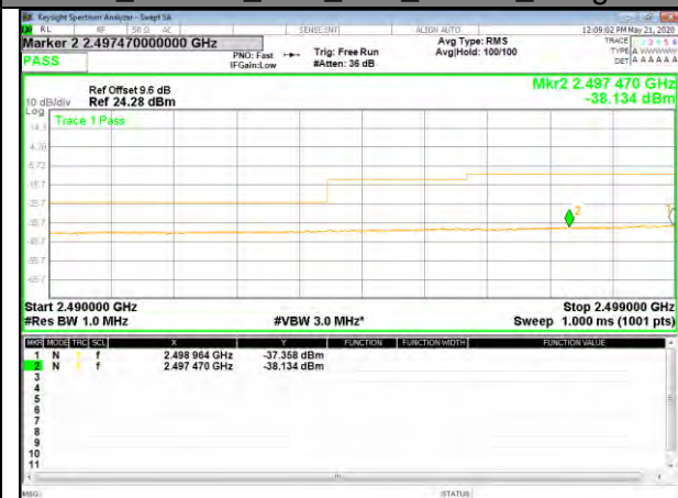
B7_16QAM_20M_Low_full-RB_Bedge
