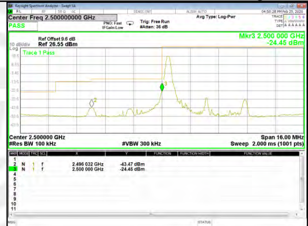
B7_16QAM_5M_Low_Full-RB_Bedge
