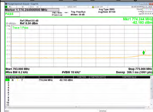
B13_16QAM_5M_Low_full-RB_Bedge
