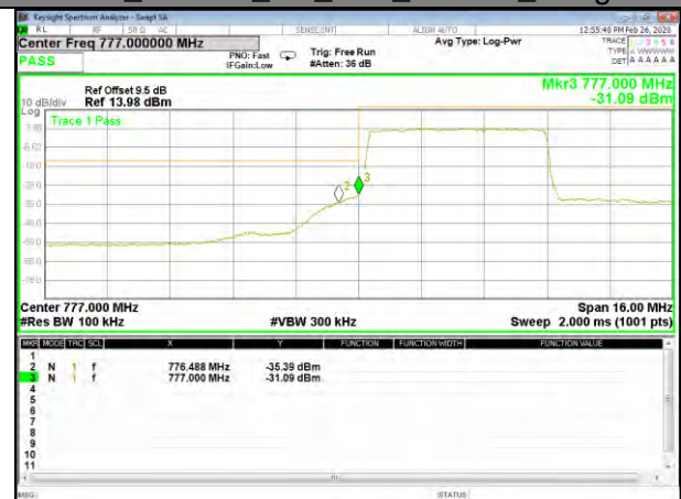
B13_16QAM_5M_Low_Full-RB_Bedge
