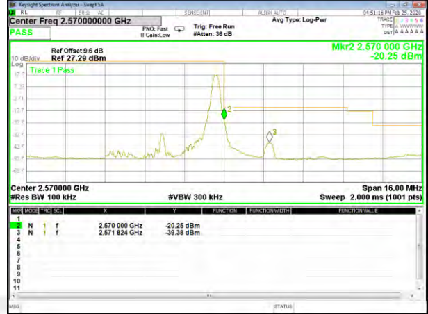
B7_16QAM_5M_High_Full-RB_Bedge
