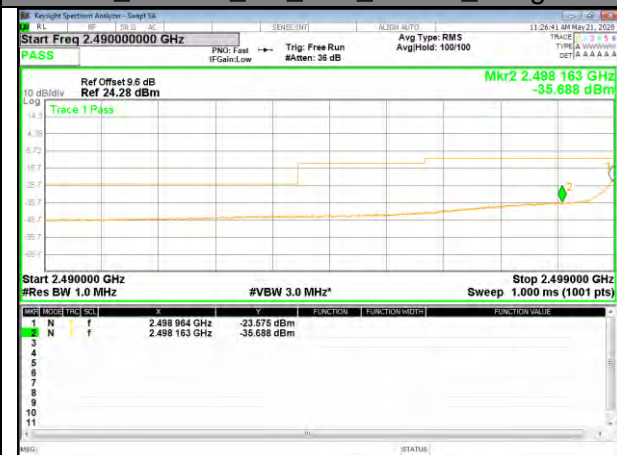
B7_16QAM_5M_Low_full-RB_Bedge
