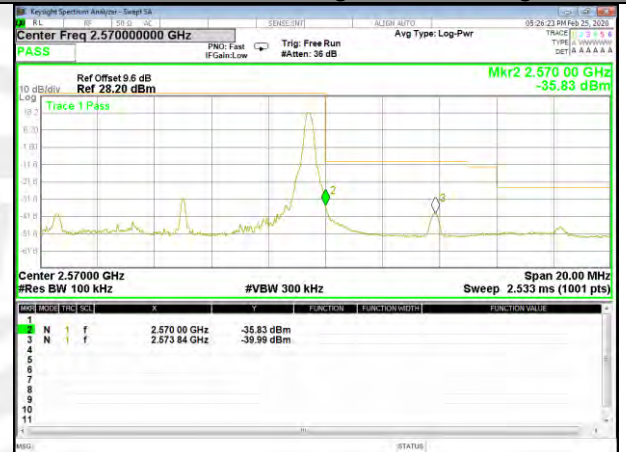
B7_QPSK_10M_High_Full-RB_Bedge
