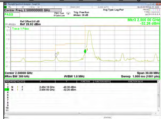
B7_16QAM_15M_Low_1-RB_Bedge
