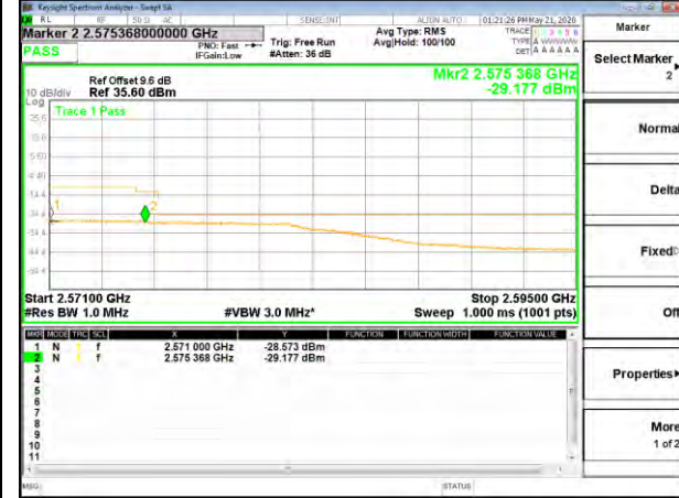
B7_16QAM_20M_High_full-RB_Bedge
