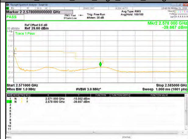
B7_16QAM_10M_High_1-RB_Bedge
