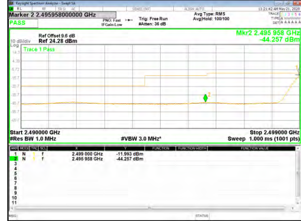
B7_QPSK_5M_Low_full-RB_Bedge
