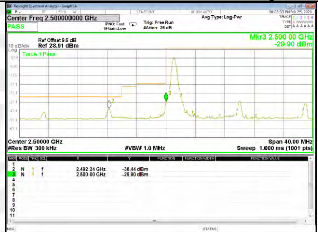
B7_16QAM_20M_Low_Full-RB_Bedge
