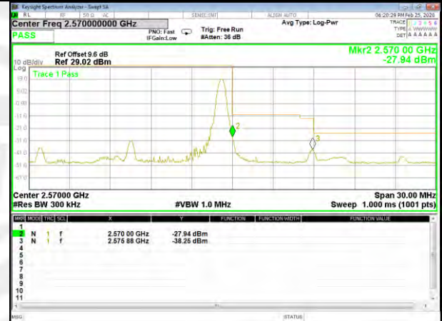
B7_16QAM_15M_High_Full-RB_Bedge
