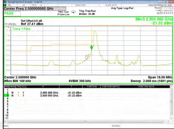
B7_QPSK_5M_Low_Full-RB_Bedge
