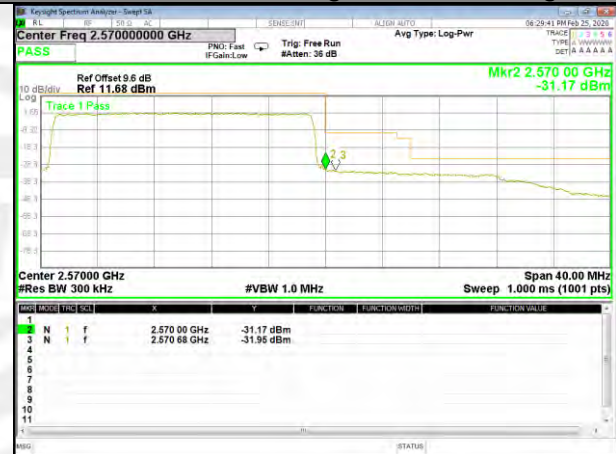
B7_16QAM_20M_High_Full-RB_Bedge
