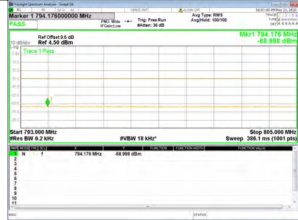
B13_16QAM_5M_High_full-RB_Bedge
