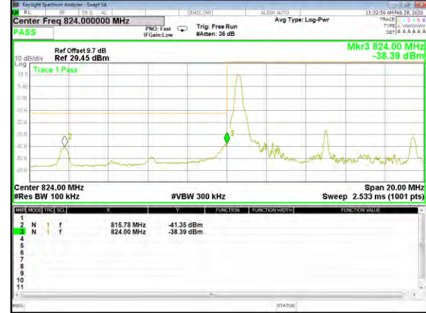
B5_QPSK_10M_High_1-RB_Bedge
