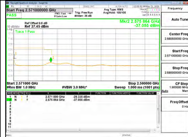
B7_16QAM_15M_High_full-RB_Bedge
