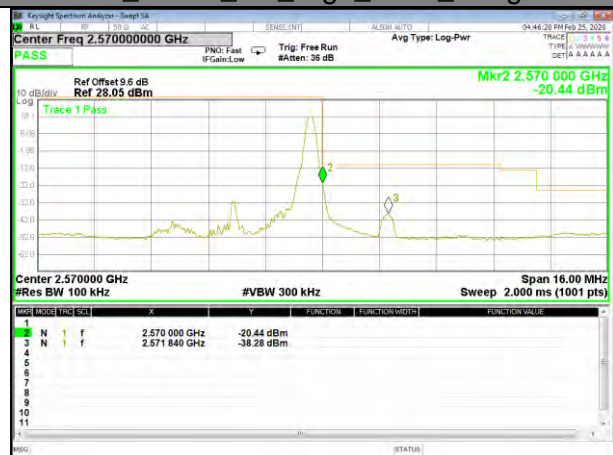
B7_QPSK_5M_High_1-RB_Bedge
