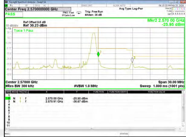
B7_QPSK_15M_High_Full-RB_Bedge
