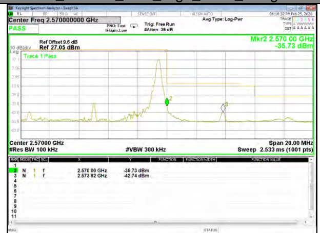
B7_16QAM_10M_High_1-RB_Bedge
