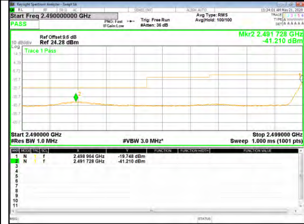
B7_16QAM_10M_Low_full-RB_Bedge
