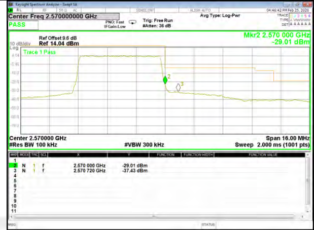
B7_16QAM_5M_Low_1-RB_Bedge
